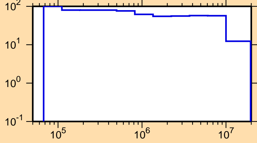
\Delta\sigma/\sigma vs. E for ^{172}\text{Ir}(n,n_1)
