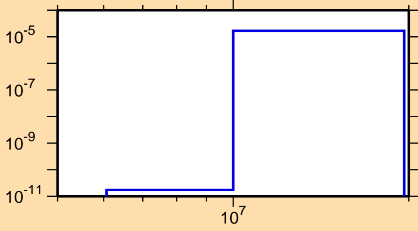
\sigma vs. E for ^{172}\text{Ir}(n,\text{pd})
