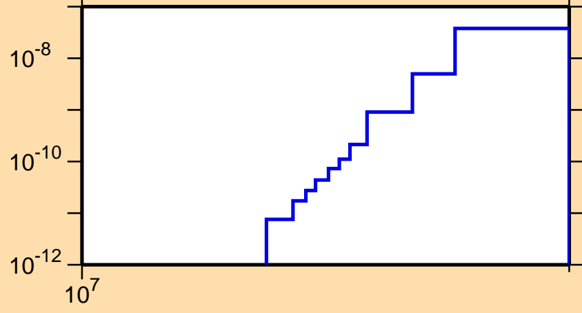
\sigma vs. E for ^{172}\text{Ir}(\text{mt } 34)
