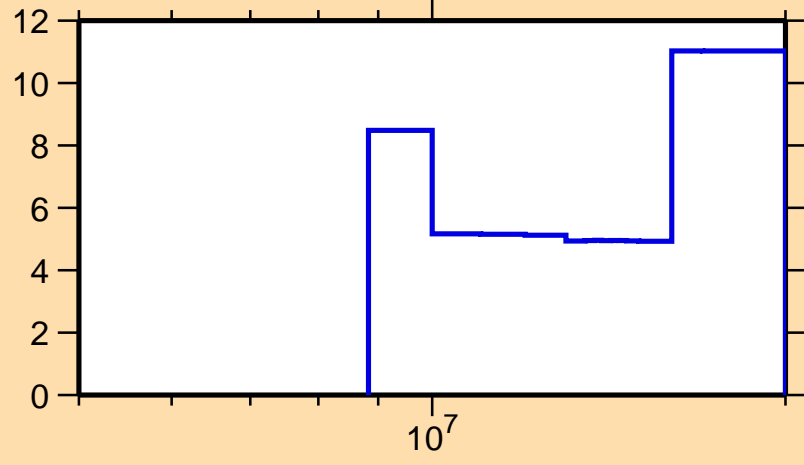
\Delta\sigma/\sigma vs. E for ^{172}\text{Ir}(n,el.)
