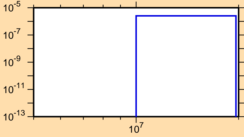
\sigma vs. E for ^{172}\text{Ir}(n,\text{nd})
