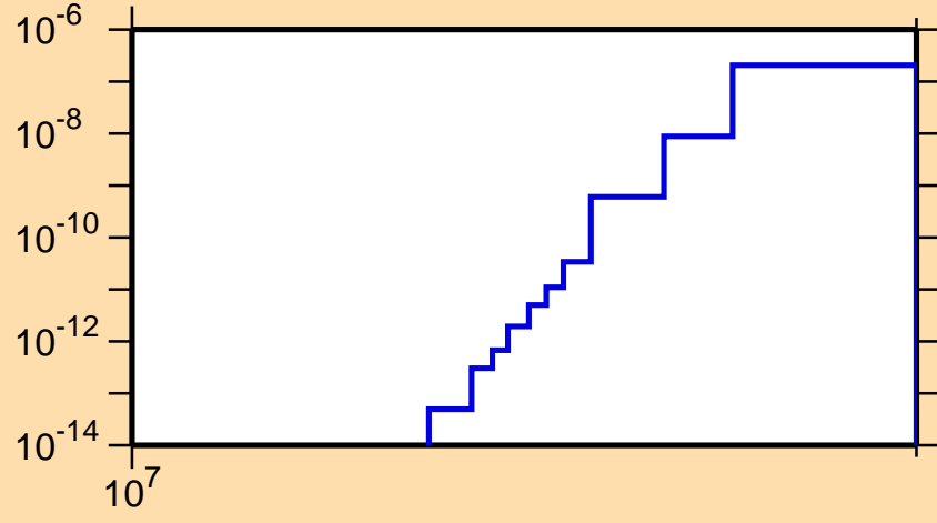
\sigma vs. E for ^{173}\text{Ir}(n,pt)
