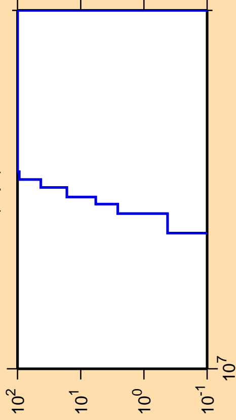
\Delta\sigma/\sigma vs. E for ^{173}\text{Ir}(n,pt)
