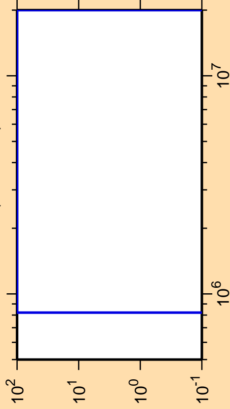
\Delta\sigma/\sigma vs. E for ^{173}\text{Ir}(n,n\text{cont.})
