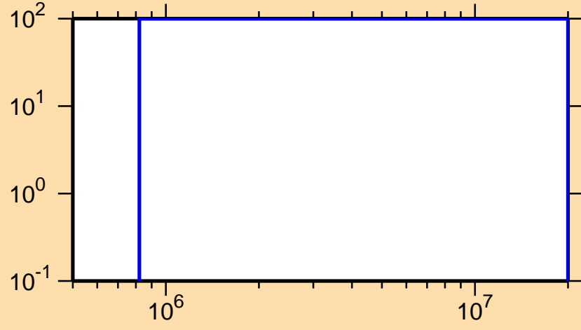
\Delta\sigma/\sigma vs. E for ^{173}\text{Ir}(n,n\text{cont.})
