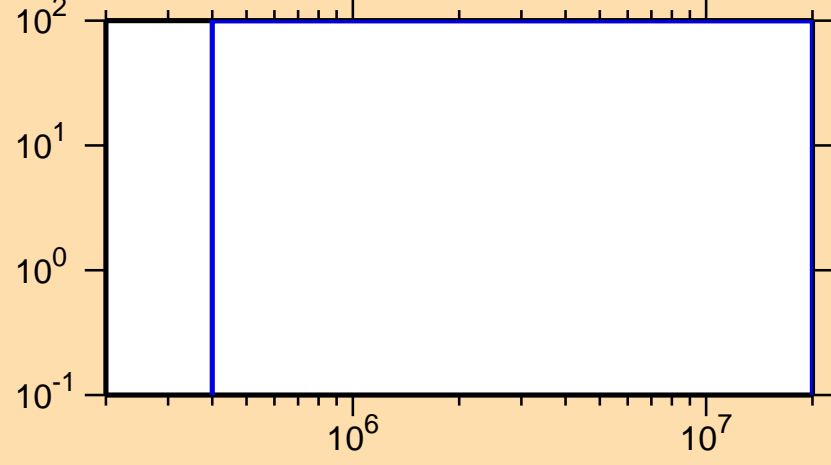
\Delta\sigma/\sigma vs. E for ^{173}\text{Ir}(n,n\text{cont.})
