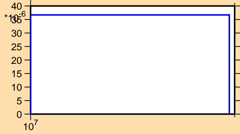
\sigma vs. E for ^{173}\text{Ir}(n,2np)
