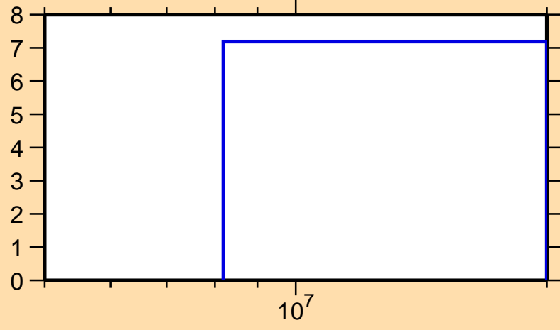
\Delta\sigma/\sigma vs. E for ^{173}\text{Ir}(n,\text{nonel.})
