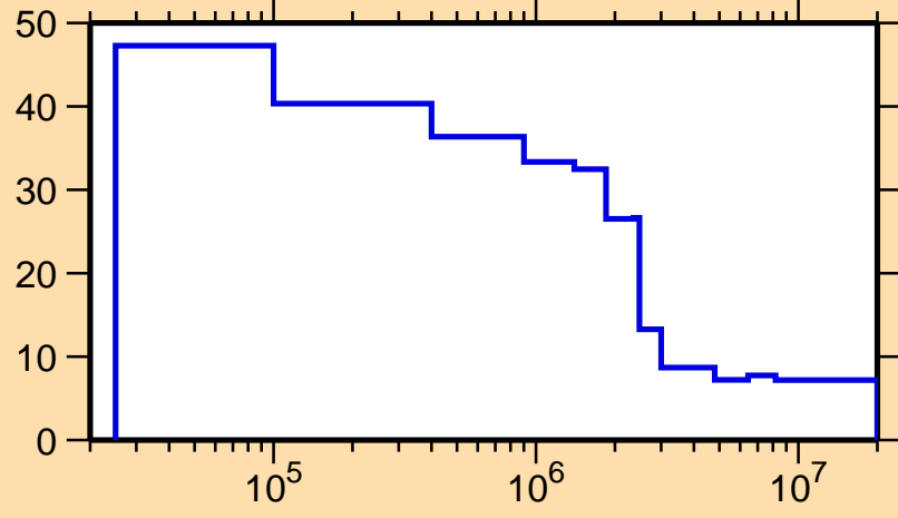
\Delta\sigma/\sigma vs. E for ^{173}\text{Ir}(n,n\text{nonel.})
