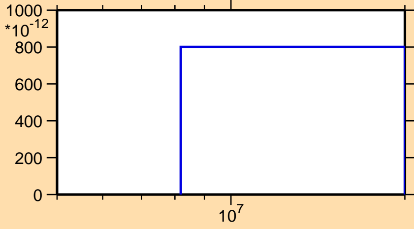
\sigma vs. E for ^{173}\text{Ir}(n,\text{pt})
