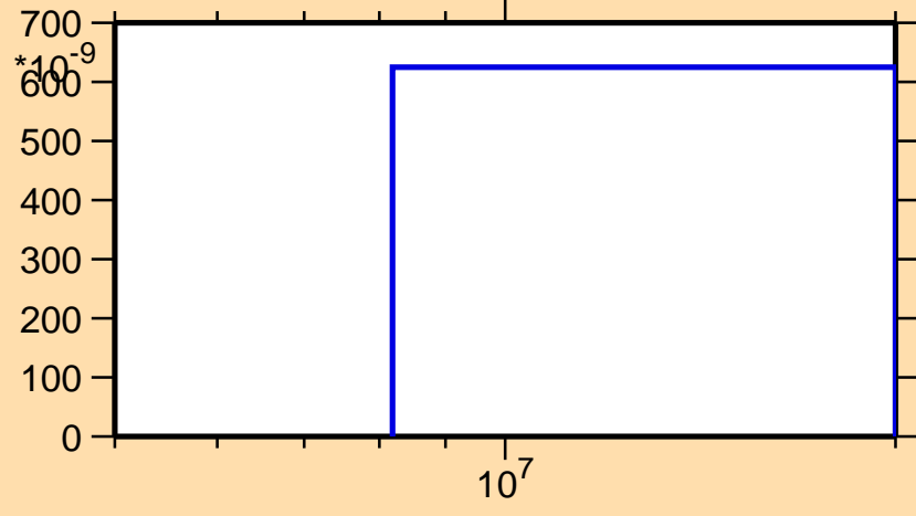
\sigma vs. E for ^{173}\text{Ir}(n,\text{pd})
