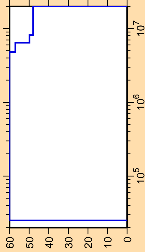
\Delta\sigma/\sigma vs. E for ^{173}\text{Ir}(n,\text{ncont.})
