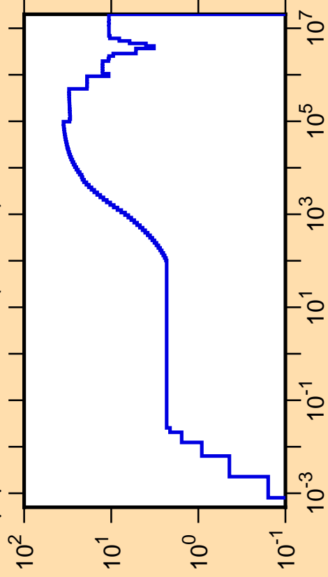
\Delta\mu/\mu vs. E for ^{174}\text{Ir}(\text{mt251})
