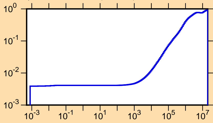
\mu vs. E for ^{174}\text{Ir}(\text{mt251})
