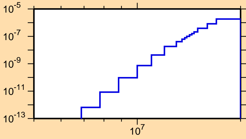
\sigma vs. E for ^{174}\text{Ir}(\text{mt117})
