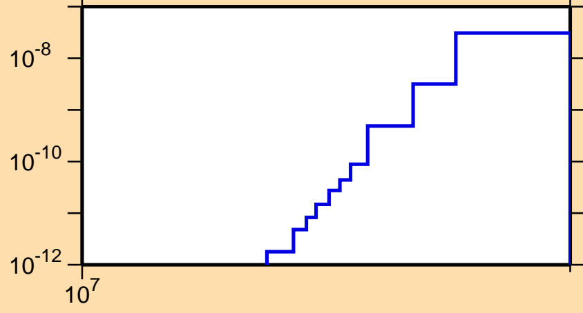
\sigma vs. E for ^{174}\text{Ir}(\text{mt } 34)
