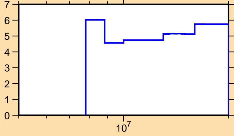
\Delta\sigma/\sigma vs. E for ^{174}\text{Ir}(n,\text{tot.})
