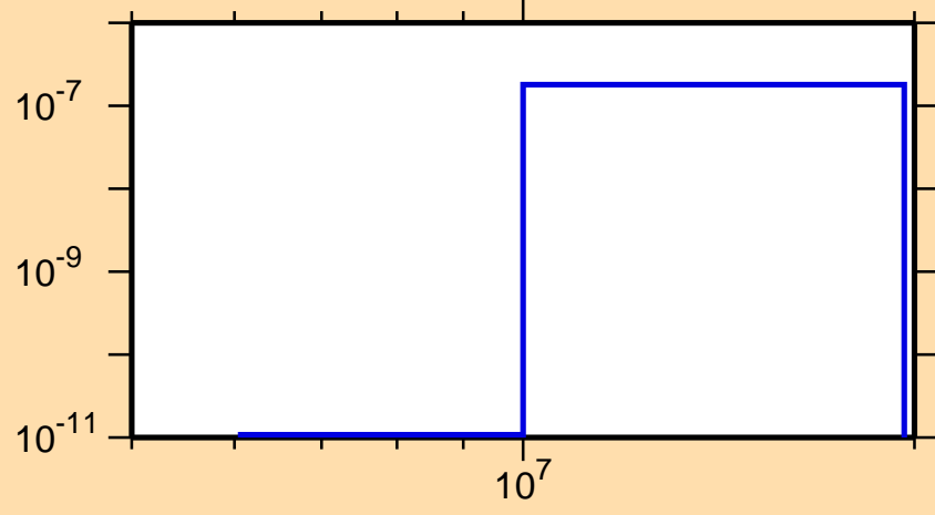
\sigma vs. E for ^{174}\text{Ir}(\text{mt117})
