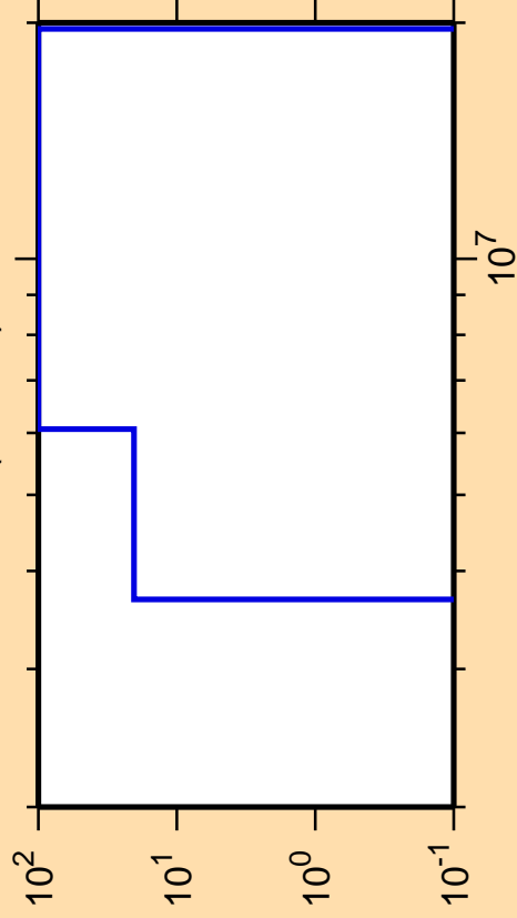
\Delta\sigma/\sigma vs. E for ^{174}\text{Ir}(n,\text{He3})
