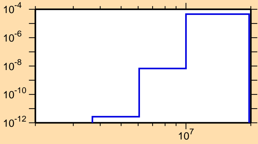
\sigma vs. E for ^{174}\text{Ir}(n,\text{He3})
