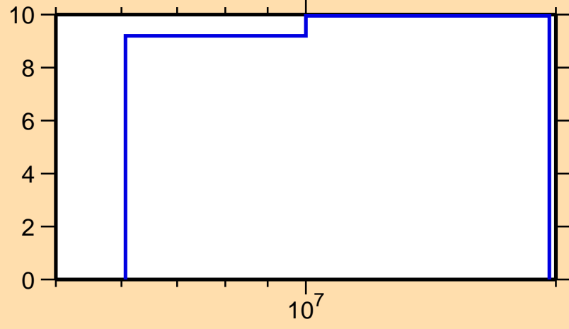
\Delta\sigma/\sigma vs. E for ^{174}\text{Ir}(n,el.)
