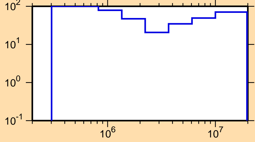
\Delta\sigma/\sigma vs. E for ^{174}\text{Ir}(n,n\text{cont.})
