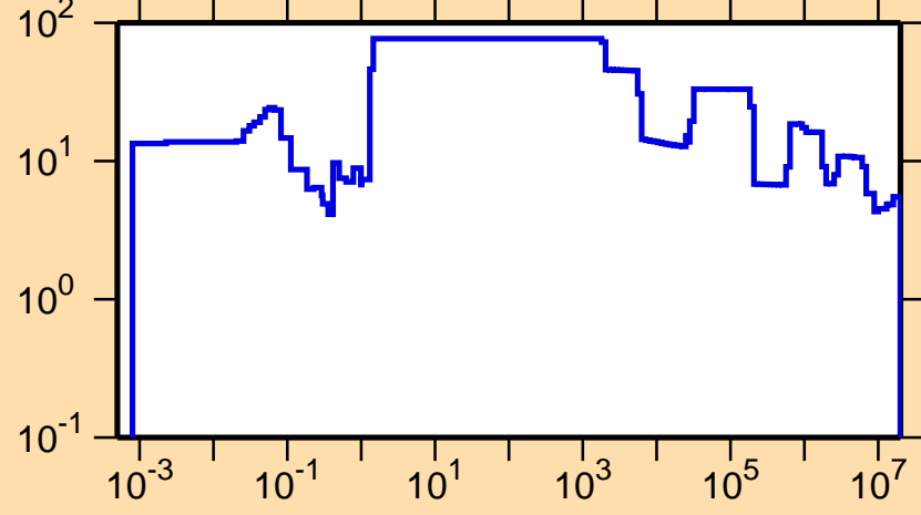
\Delta\sigma/\sigma vs. E for ^{174}\text{Ir}(n,\text{tot.})
