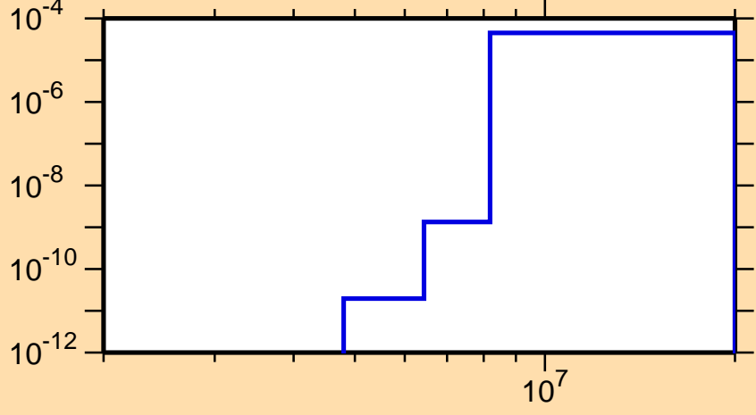
\sigma vs. E for ^{174}\text{Ir}(n,\text{He}3)
