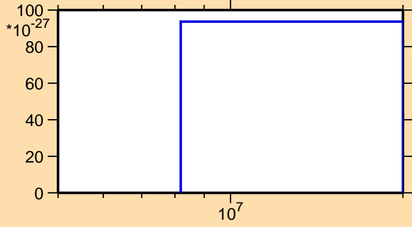
\sigma vs. E for ^{174}\text{Ir}(\text{mt } 42)
