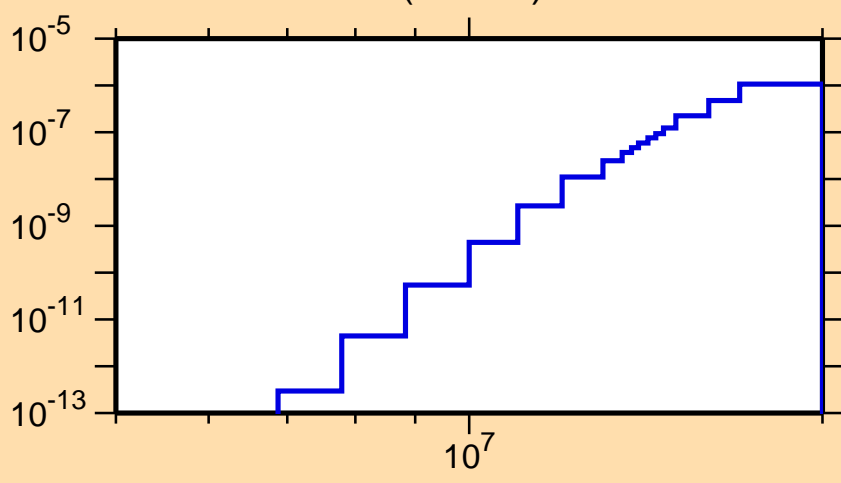
\sigma vs. E for ^{175}\text{Ir}(\text{mt117})
