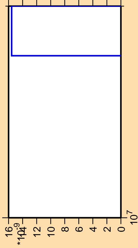
\Delta\sigma/\sigma vs. E for ^{175}\text{Ir} (mt 42)
