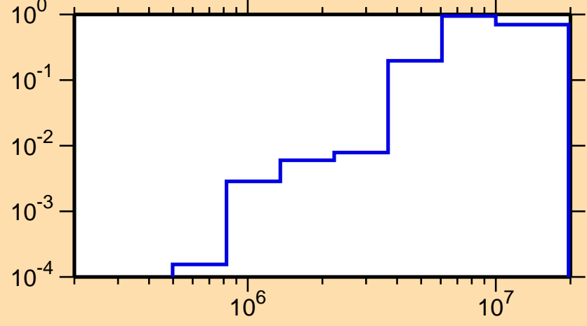
\sigma vs. E for ^{175}\text{Ir}(n,n\text{cont.})
