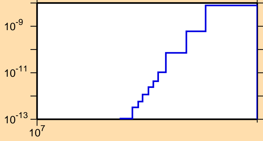
\sigma vs. E for ^{176}\text{Ir}(\text{mt } 34)
