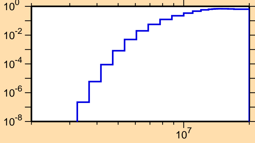
\sigma vs. E for ^{176}\text{Ir}(n,np)
