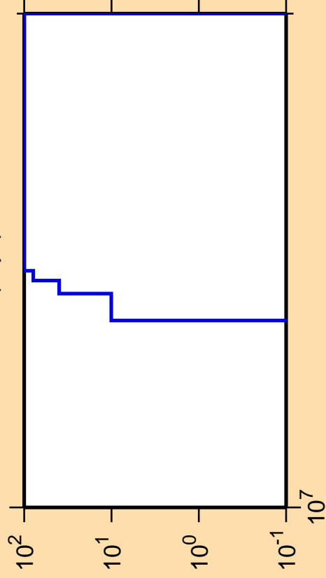
\Delta\sigma/\sigma vs. E for ^{176}\text{Ir}(n,pt)
