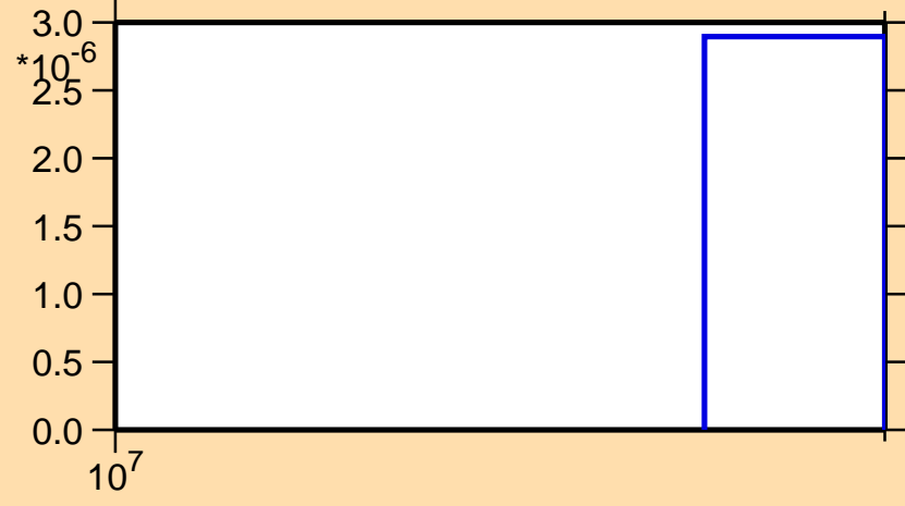
\sigma vs. E for ^{176}\text{Ir}(n,3n)
