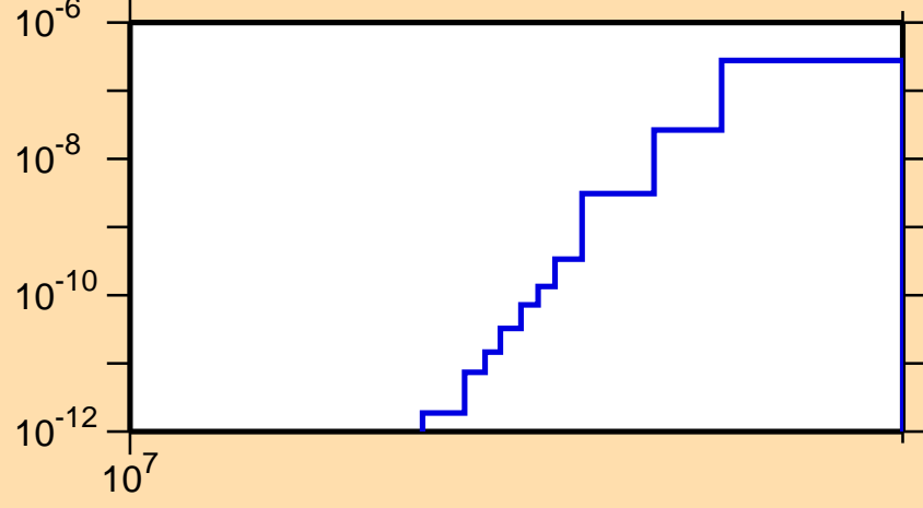
\sigma vs. E for ^{176}\text{Ir}(n,pt)
