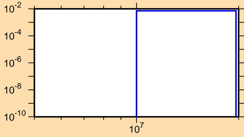
\sigma vs. E for ^{176}\text{Ir}(n,2np)
