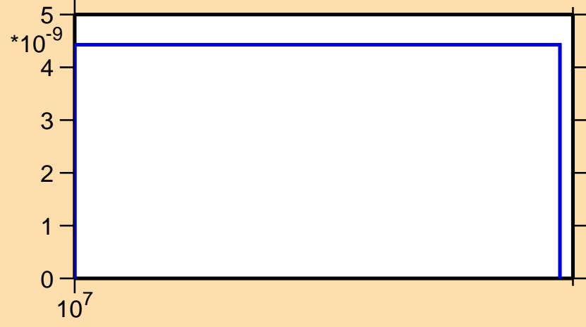
\sigma vs. E for ^{176}\text{Ir}(n,\text{pt})
