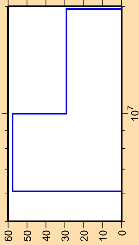
\Delta\sigma/\sigma vs. E for ^{176}\text{Ir}(n,p)
