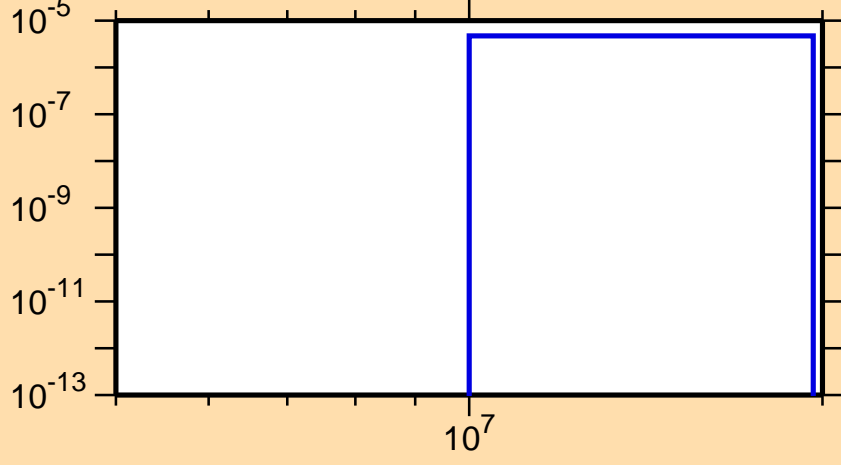
\sigma vs. E for ^{176}\text{Ir}(n,\text{nd})
