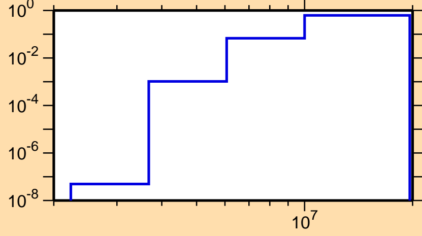
\sigma vs. E for ^{176}\text{Ir}(n,np)
