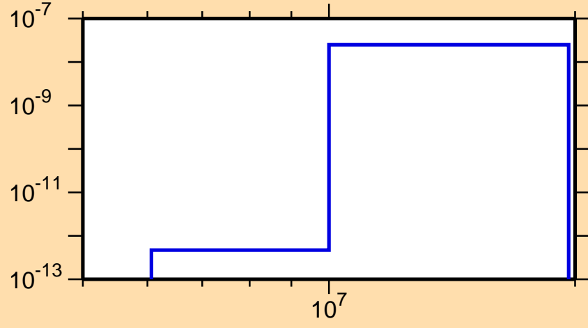
\sigma vs. E for ^{176}\text{Ir}(\text{mt117})
