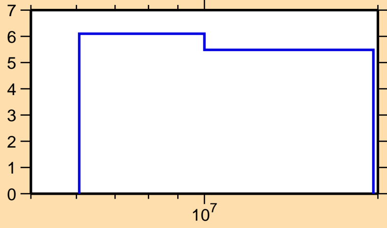
\Delta\sigma/\sigma vs. E for ^{176}\text{Ir}(n,\text{nonel.})
