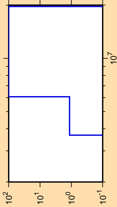
\Delta\sigma/\sigma vs. E for ^{176}\text{Ir}(n,\text{He}3)
