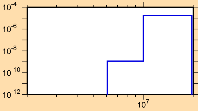
\sigma vs. E for ^{176}\text{Ir}(n,\text{He}3)
