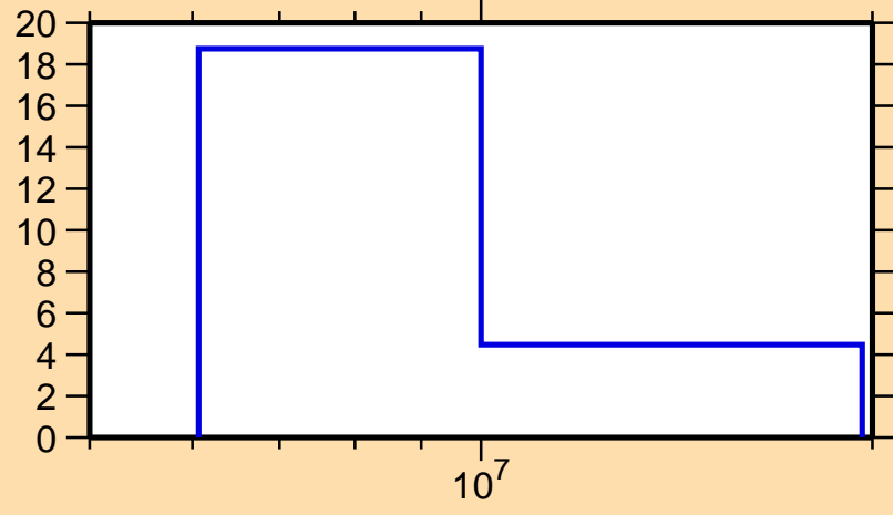
\Delta\sigma/\sigma vs. E for ^{176}\text{Ir}(n,\text{el.})
