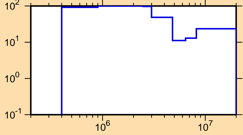
\Delta\sigma/\sigma vs. E for ^{177}\text{Ir}(n,ncont.)
