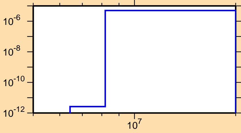
\sigma vs. E for ^{177}\text{Ir}(\text{mt } 45)
