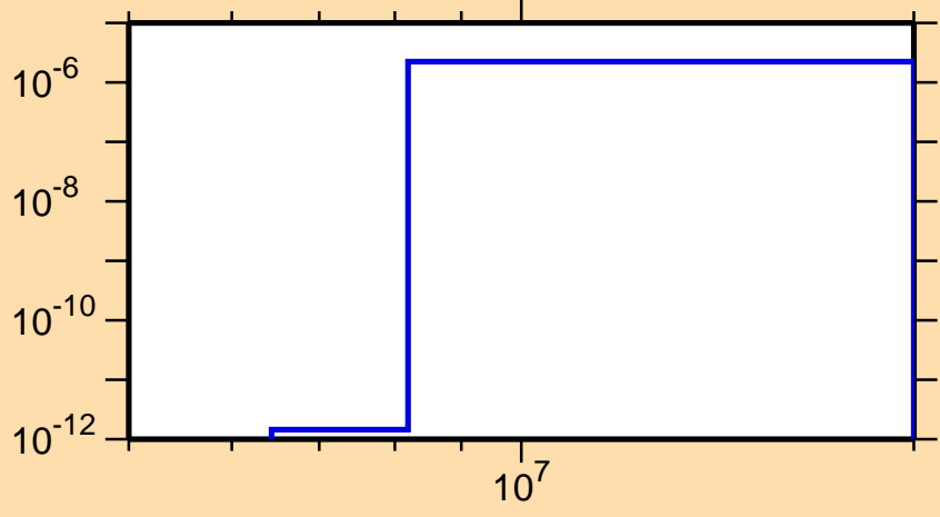
\sigma vs. E for ^{177}\text{Ir}(n,\text{He}3)
