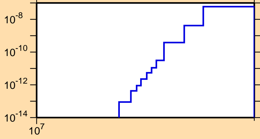
\sigma vs. E for ^{178}\text{Ir}(n,\text{pt})
