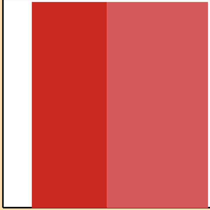
\Delta\sigma/\sigma vs. E for ^{178}\text{Ir}(n,2n)
