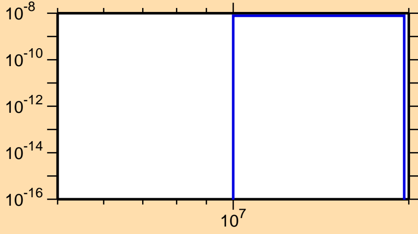
\sigma vs. E for ^{178}\text{Ir}(n,\text{pd})
