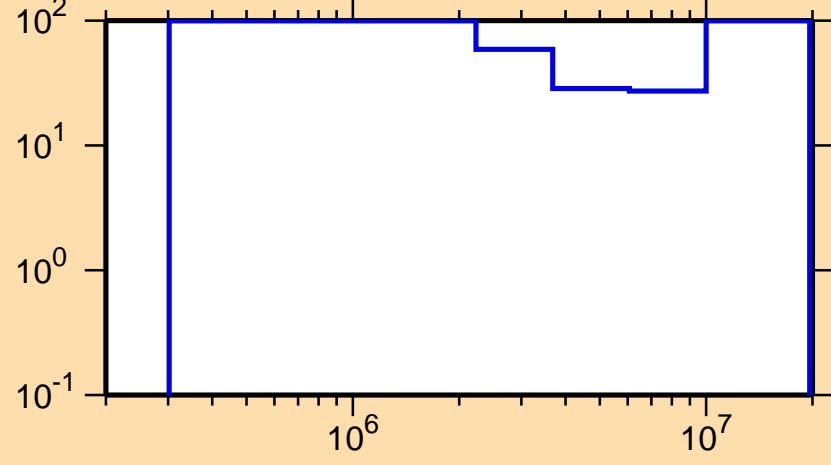
\Delta\sigma/\sigma vs. E for ^{178}\text{Ir}(n,n\text{cont.})
