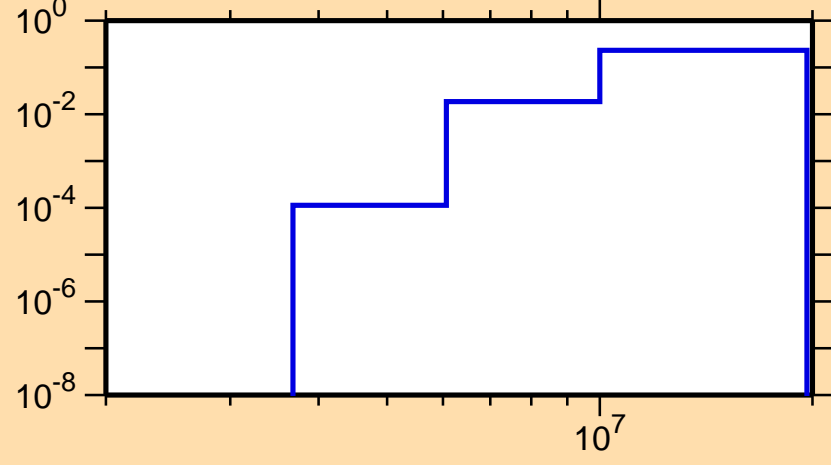
\sigma vs. E for ^{178}\text{Ir}(n,np)
