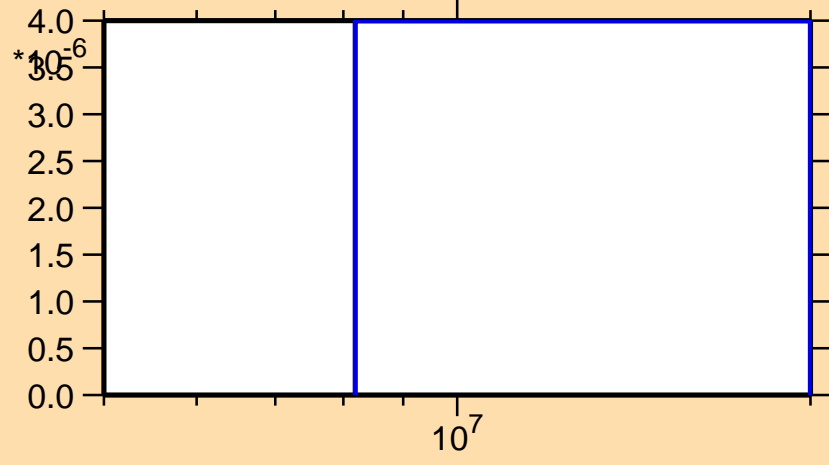
\sigma vs. E for ^{178}\text{Ir}(n,\text{nd})
