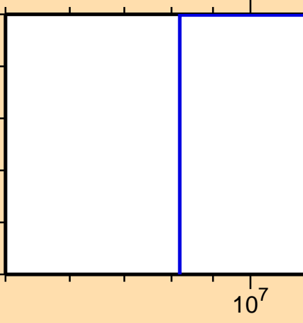
\sigma vs. E for ^{178}\text{Ir}(\text{mt117})
