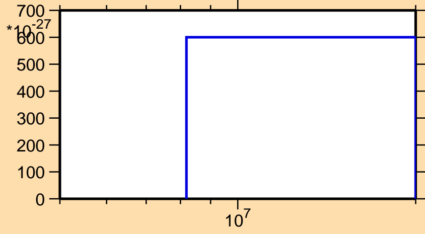
\sigma vs. E for ^{178}\text{Ir}(\text{mt } 42)
