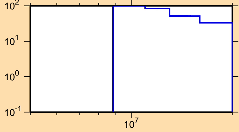
\Delta\sigma/\sigma vs. E for ^{179}\text{Ir}(n,2n)
