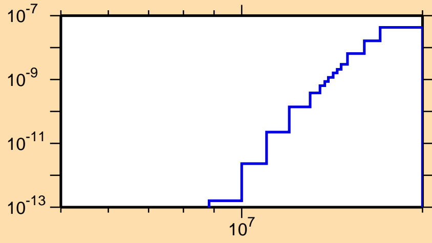
\sigma vs. E for ^{179}\text{Ir}(\text{mt117})
