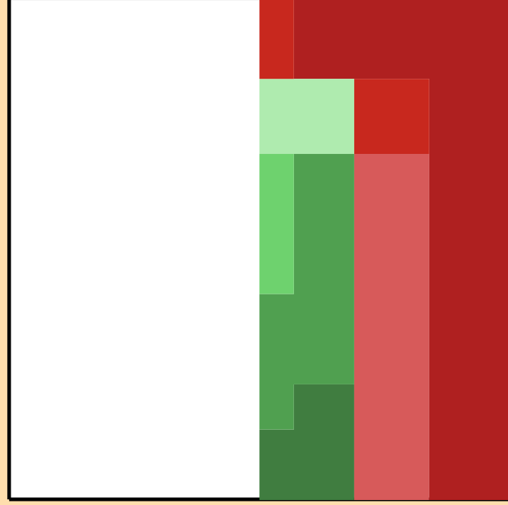
\Delta\sigma/\sigma vs. E for ^{179}\text{Ir}(n,2n)
