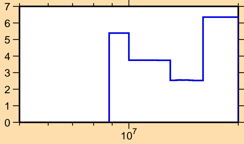
\Delta\sigma/\sigma vs. E for ^{179}\text{Ir}(n,\text{tot.})
