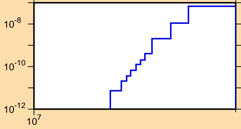
\sigma vs. E for ^{179}\text{Ir}(n,\text{pd})
