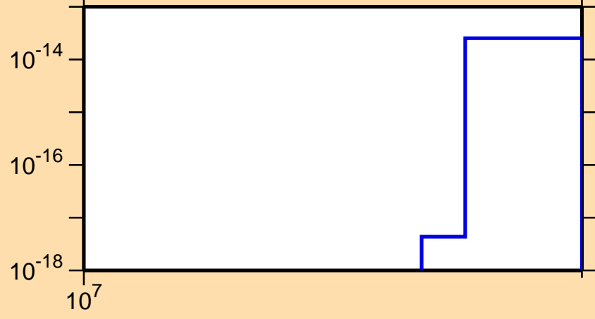
\sigma vs. E for ^{179}\text{Ir}(n,3n\alpha)
