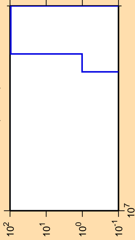
\Delta\sigma/\sigma vs. E for ^{179}\text{Ir} (mt 34)
