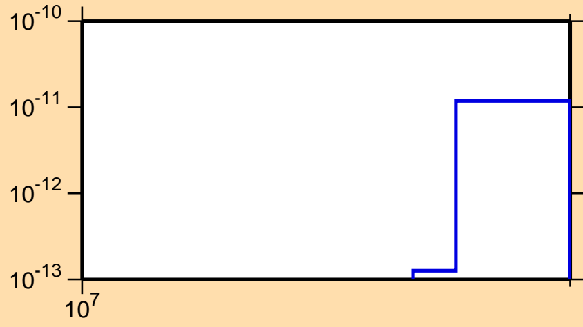
\sigma vs. E for ^{179}\text{Ir} (mt 34)
