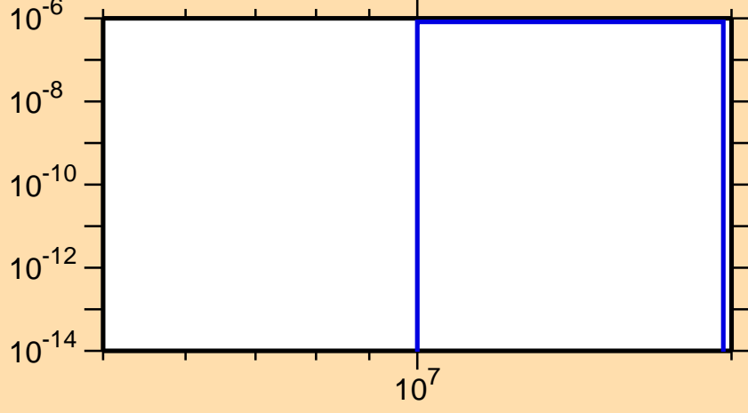
\sigma vs. E for ^{179}\text{Ir}(n,2n\alpha)
