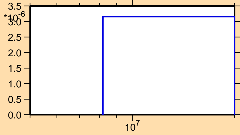
\sigma vs. E for ^{179}\text{Ir}(n,3n)
