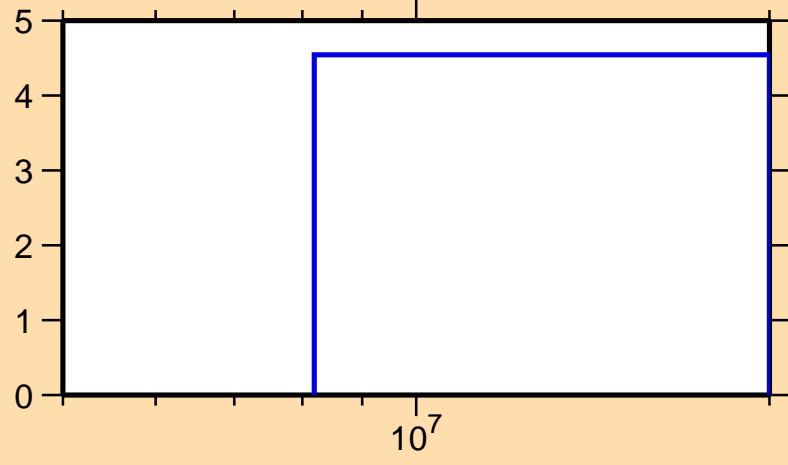
\Delta\sigma/\sigma vs. E for ^{179}\text{Ir}(n,\text{el.})
