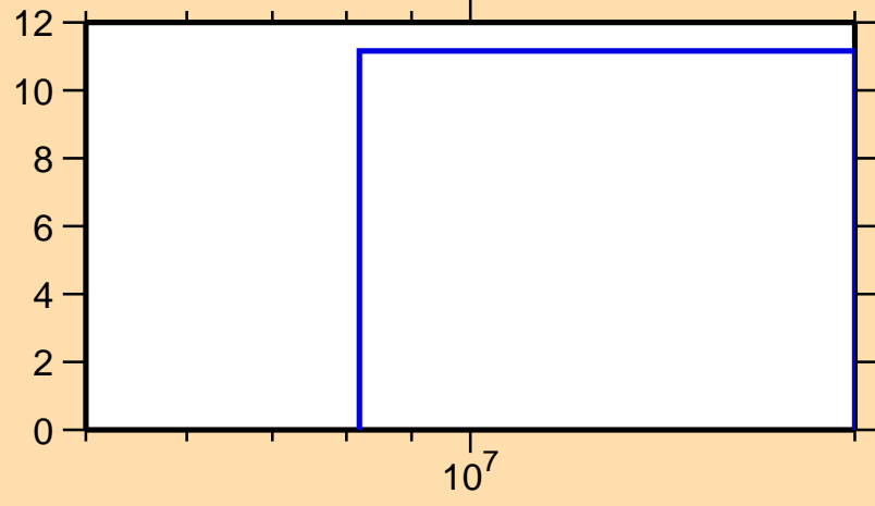
\Delta\sigma/\sigma vs. E for ^{179}\text{Ir}(n,\text{nonel.})
