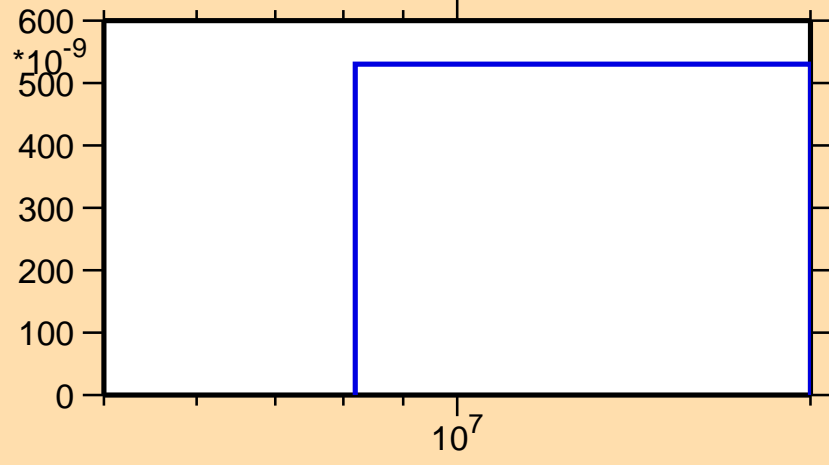
\sigma vs. E for ^{179}\text{Ir}(n,\text{He}3)
