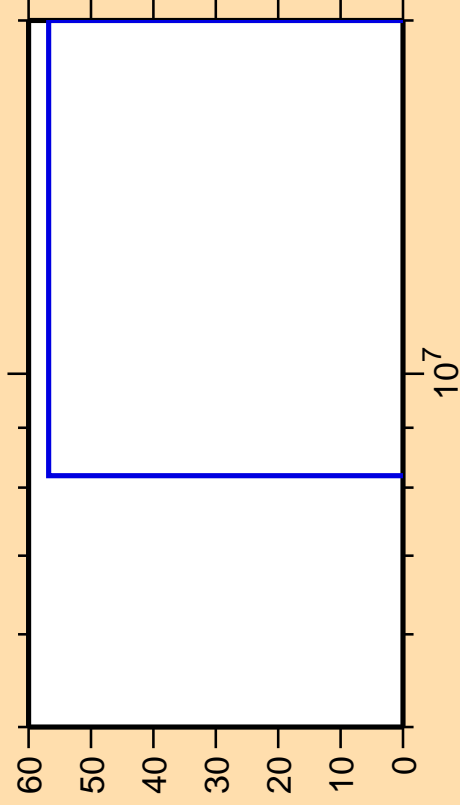
\Delta\sigma/\sigma vs. E for ^{179}\text{Ir}(n,n\text{cont.})
