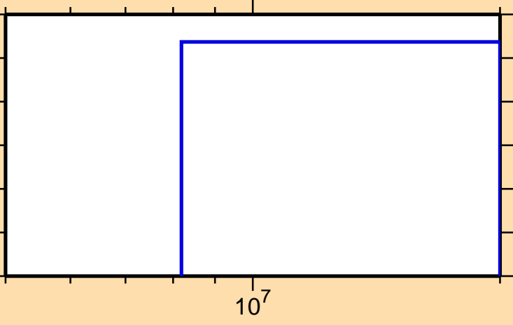
\sigma vs. E for ^{179}\text{Ir} (mt 42)
