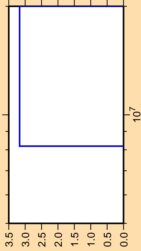
\Delta\sigma/\sigma vs. E for ^{179}\text{Ir}(n,\text{pt})
