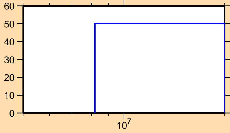
\Delta\sigma/\sigma vs. E for ^{179}\text{Ir}(n,2n)
