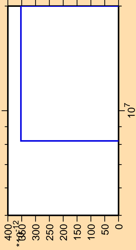
\Delta\sigma/\sigma vs. E for ^{179}\text{Ir} (mt 42)
