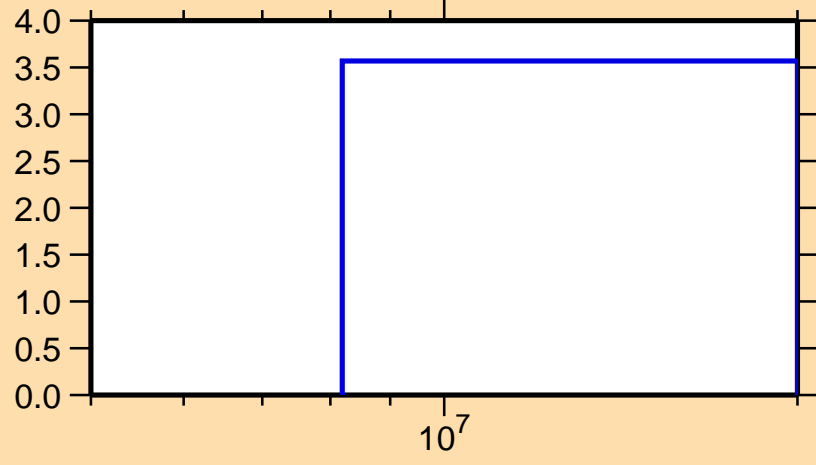
\Delta\sigma/\sigma vs. E for ^{179}\text{Ir}(n,\text{tot.})
