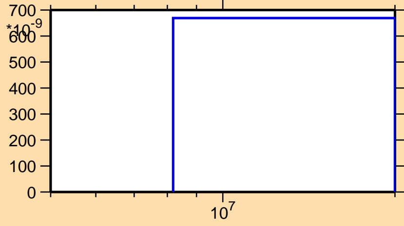
\sigma vs. E for ^{179}\text{Ir}(n,2n\alpha)
