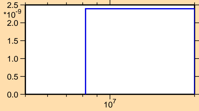
\sigma vs. E for ^{179}\text{Ir}(\text{mt117})
