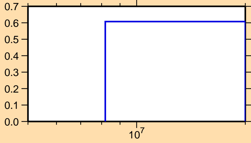
\sigma vs. E for ^{179}\text{Ir}(n,2n)
