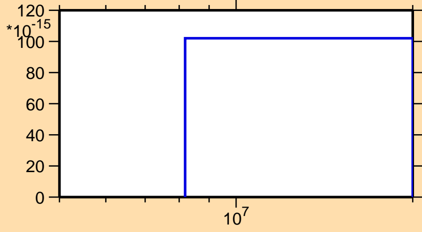
\sigma vs. E for ^{179}\text{Ir}(\text{mt } 34)
