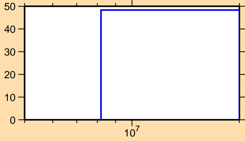
\Delta\sigma/\sigma vs. E for ^{179}\text{Ir}(n,\text{inel.})
