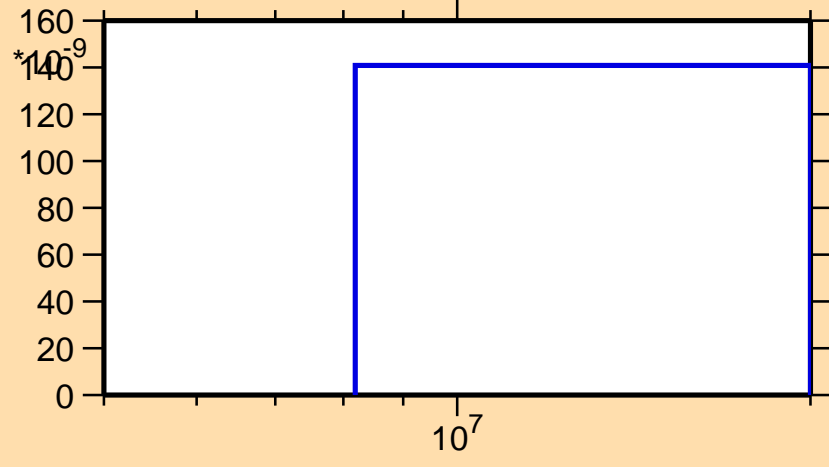
\sigma vs. E for ^{179}\text{Ir}(n,\text{nd})
