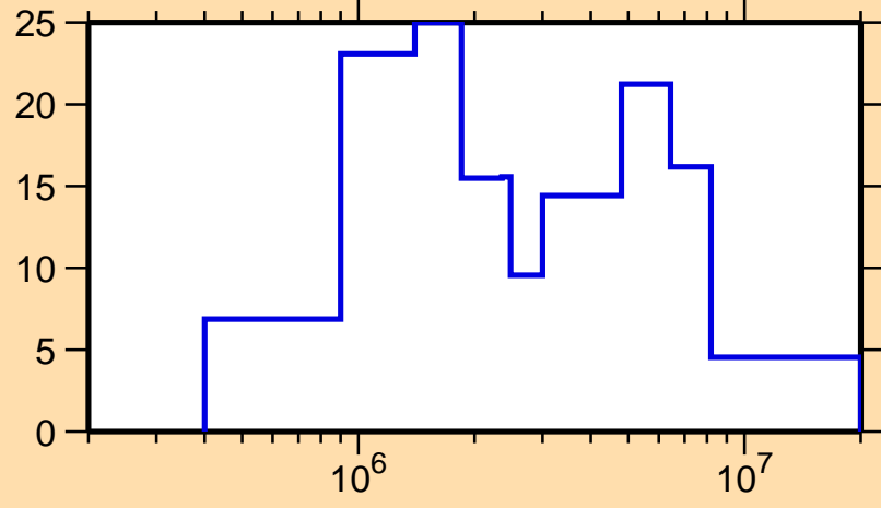
\Delta\sigma/\sigma vs. E for ^{179}\text{Ir}(n,el.)
