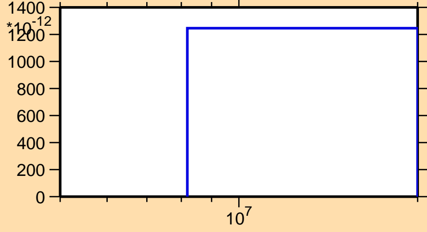
\sigma vs. E for ^{179}\text{Ir}(n,nt)
