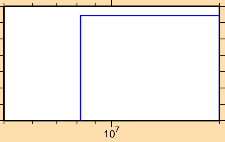
\sigma vs. E for ^{179}\text{Ir}(n,\text{pd})
