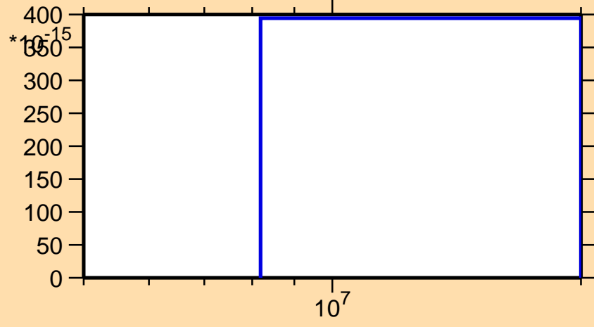
\sigma vs. E for ^{179}\text{Ir}(n,\text{pt})
