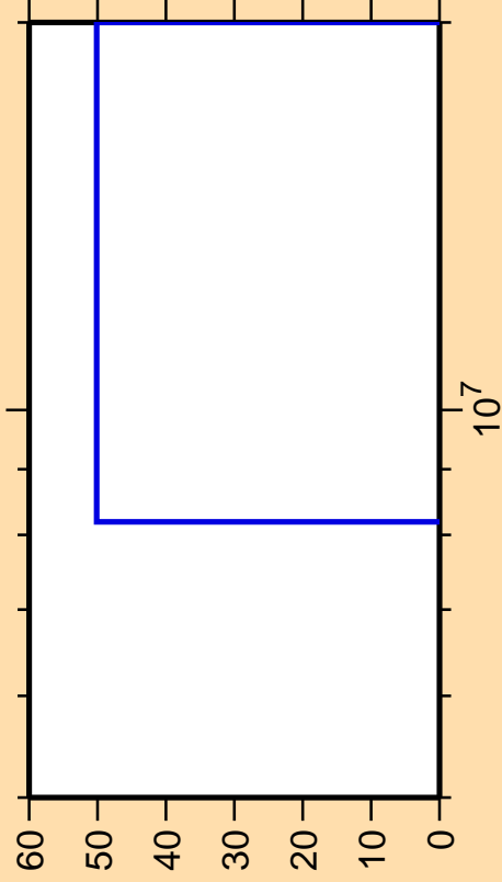
\Delta\sigma/\sigma vs. E for ^{179}\text{Ir}(n,2n)
