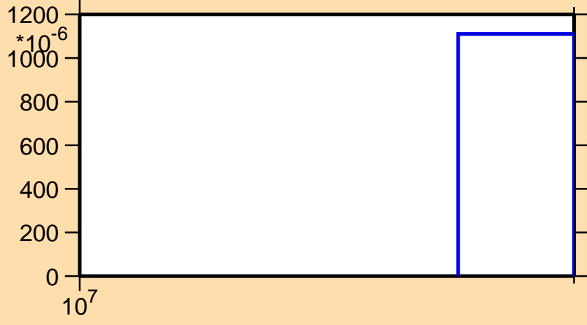
\sigma vs. E for ^{180}\text{Ir}(n,3n)
