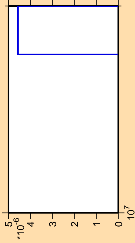
\Delta\sigma/\sigma vs. E for ^{180}\text{Ir} (mt 42)
