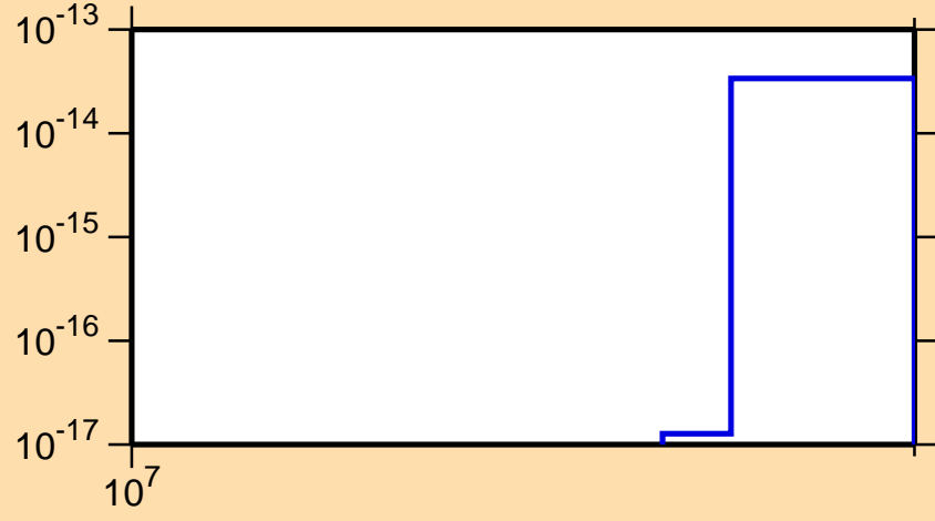
\sigma vs. E for ^{180}\text{Ir}(n,3n\alpha)
