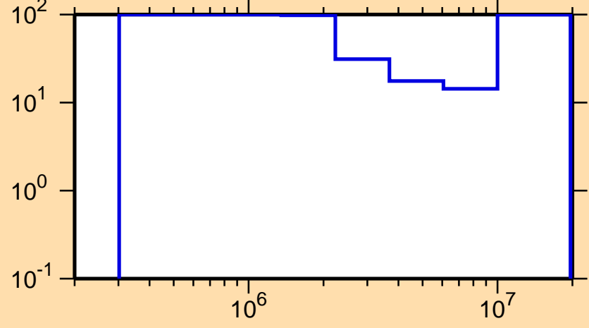
\Delta\sigma/\sigma vs. E for ^{180}\text{Ir}(n,n\text{cont.})
