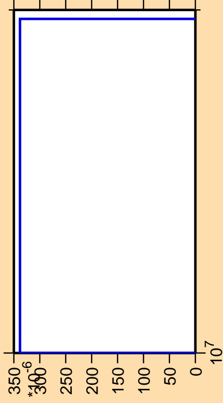
\Delta\sigma/\sigma vs. E for ^{180}\text{Ir}(n,3n\alpha)
