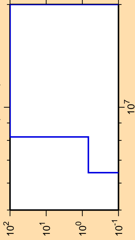
\Delta\sigma/\sigma vs. E for ^{180}\text{Ir}(n,\text{He}3)
