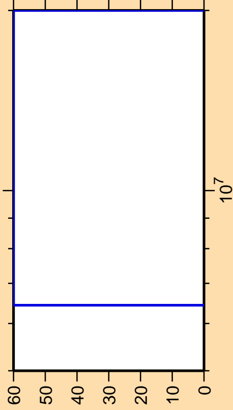
\Delta\sigma/\sigma vs. E for ^{180}\text{Ir}(n,n_1)
