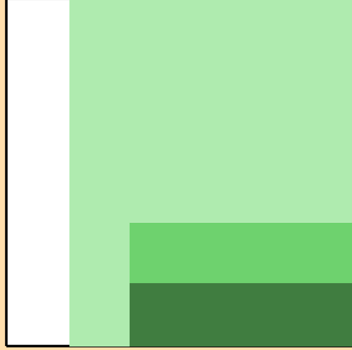
\Delta\sigma/\sigma vs. E for ^{180}\text{Ir}(n,2n)
