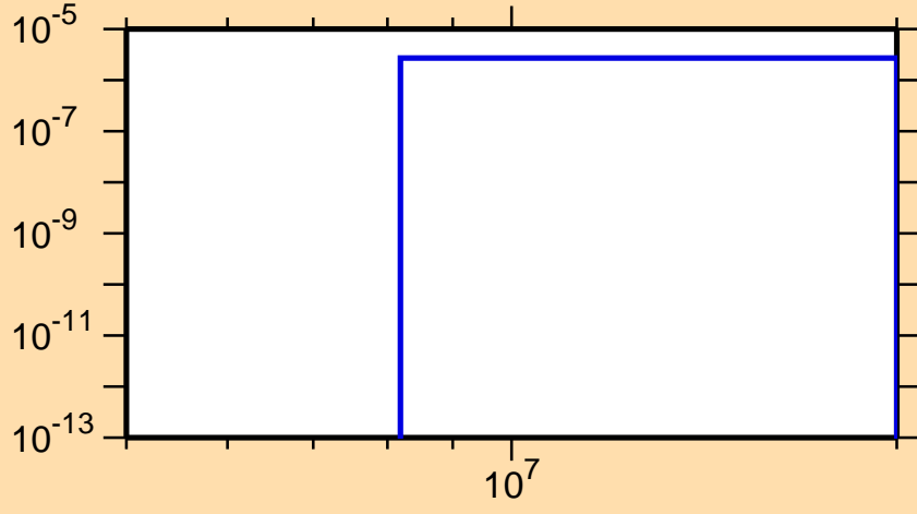
\sigma vs. E for ^{180}\text{Ir}(n,\text{nd})
