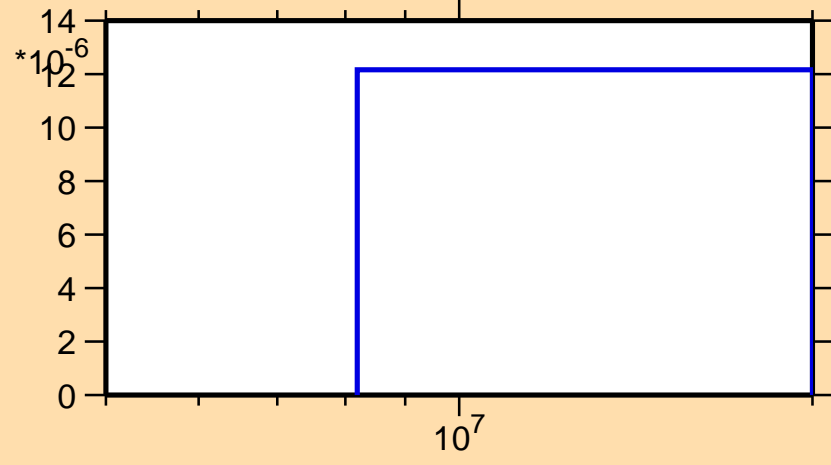
\sigma vs. E for ^{180}\text{Ir}(n,2n\alpha)
