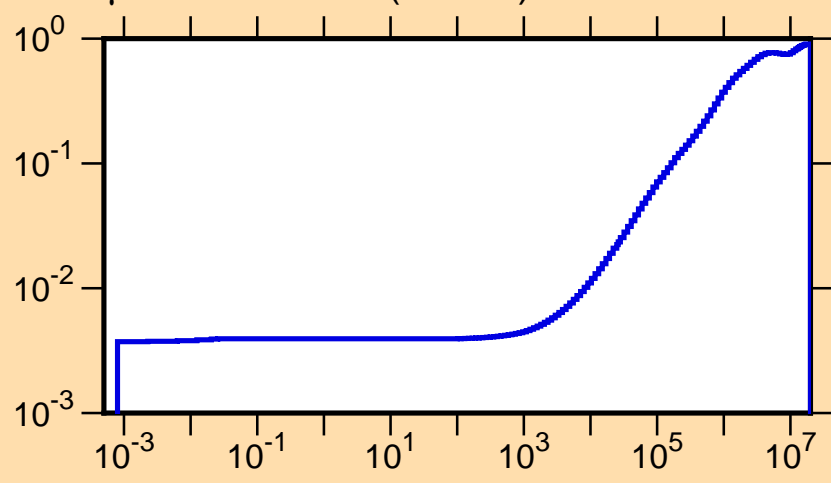
\mu vs. E for ^{181}\text{Ir}(\text{mt251})
