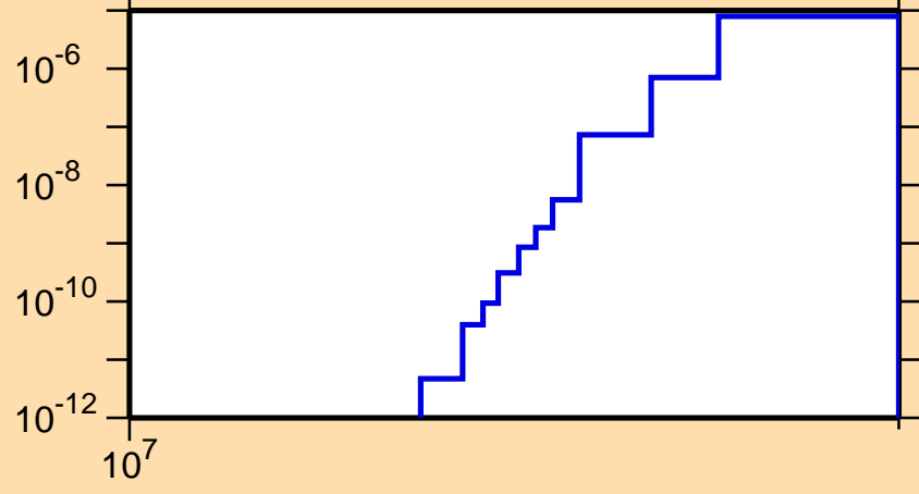
\sigma vs. E for ^{181}\text{Ir}(n,\text{nd})
