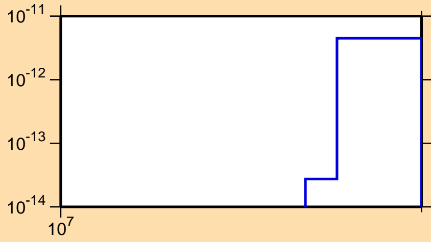
\sigma vs. E for ^{181}\text{Ir} (mt 34)
