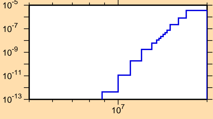
\sigma vs. E for ^{181}\text{Ir}(n,\text{He}3)
