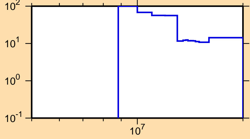
\Delta\sigma/\sigma vs. E for ^{181}\text{Ir}(n,2n)
