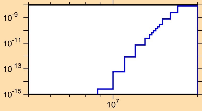
\sigma vs. E for ^{181}\text{Ir}(\text{mt117})
