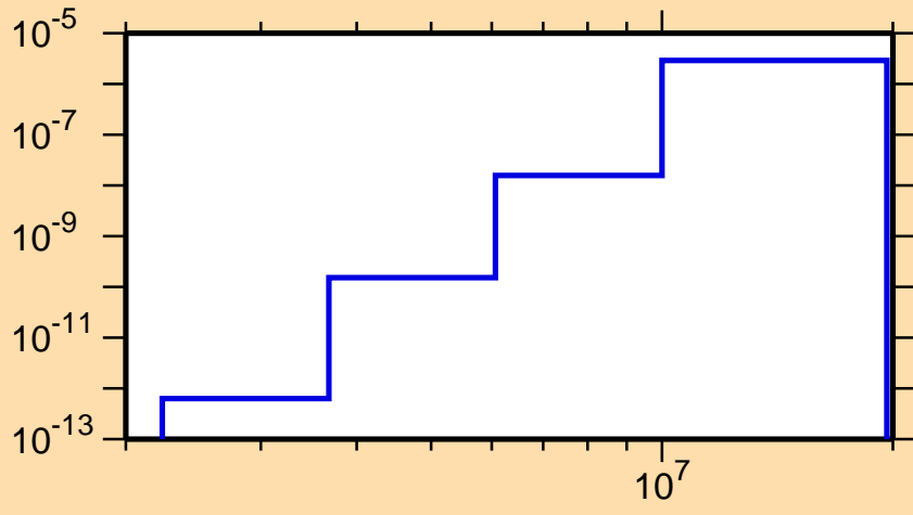
\sigma vs. E for ^{181}\text{Ir}(n,p\alpha)
