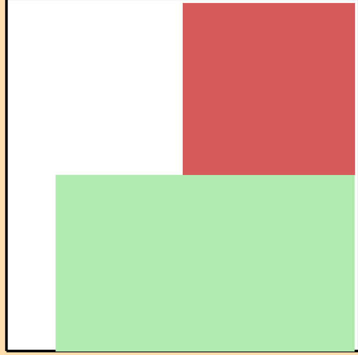
\Delta\sigma/\sigma vs. E for ^{181}\text{Ir}(n,2n)
