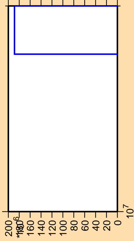
\Delta\sigma/\sigma vs. E for ^{182}\text{Ir} (mt 42)
