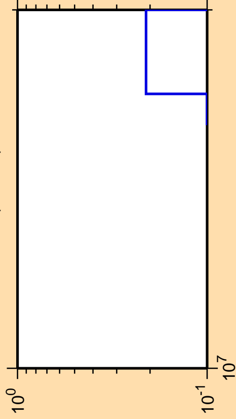
\Delta\sigma/\sigma vs. E for ^{182}\text{Ir}(n,3n\alpha)
