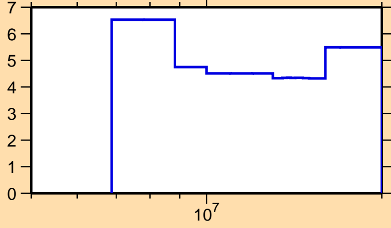
\Delta\sigma/\sigma vs. E for ^{182}\text{Ir}(n,\text{tot.})
