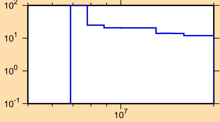
\Delta\sigma/\sigma vs. E for ^{182}\text{Ir}(n,2n)
