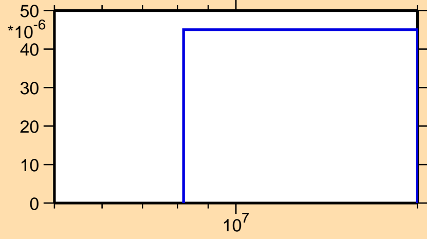
\sigma vs. E for ^{182}\text{Ir}(n,3n)
