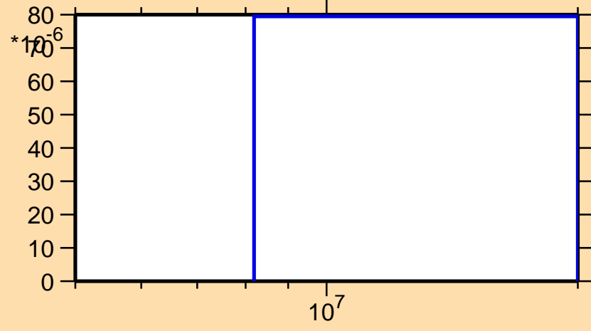
\sigma vs. E for ^{182}\text{Ir}(n,2np)
