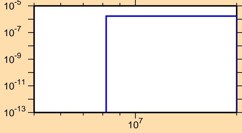
\sigma vs. E for ^{182}\text{Ir}(n,\text{nd})
