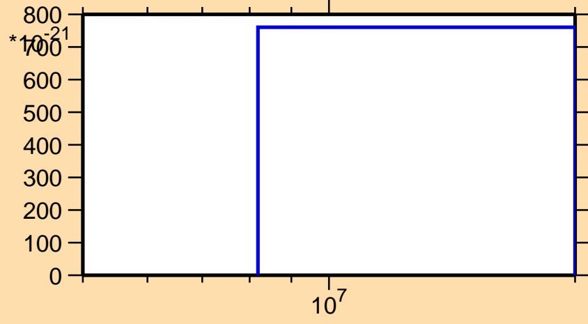
\sigma vs. E for ^{182}\text{Ir} (mt 42)
