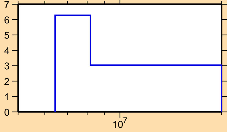
\Delta\sigma/\sigma vs. E for ^{182}\text{Ir}(n,\text{el.})
