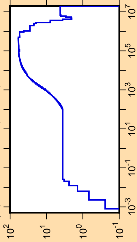
\Delta\mu/\mu vs. E for ^{183}\text{Ir}(\text{mt251})
