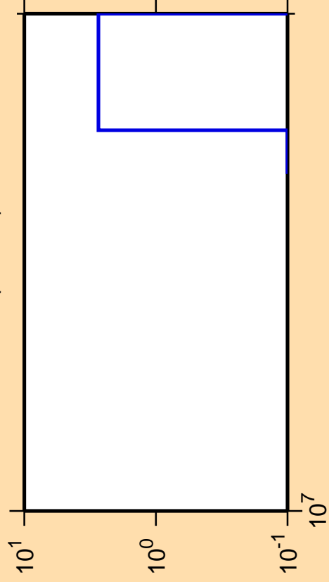
\Delta\sigma/\sigma vs. E for ^{183}\text{Ir} (mt 34)
