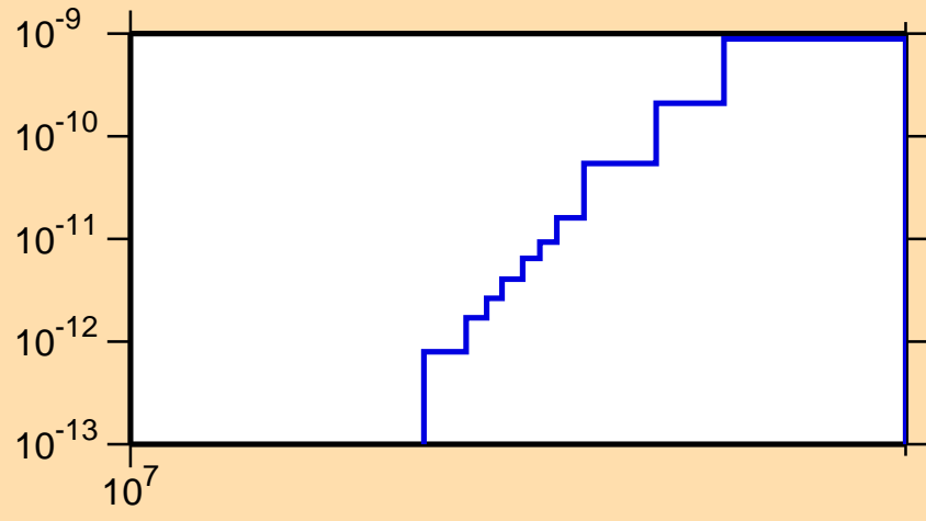
\sigma vs. E for ^{183}\text{Ir}(\text{mt117})
