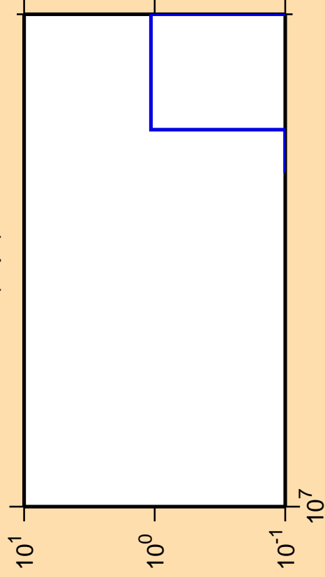
\Delta\sigma/\sigma vs. E for ^{183}\text{Ir}(n,\text{pt})
