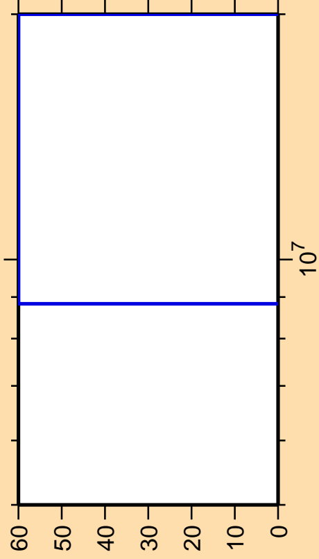
\Delta\sigma/\sigma vs. E for ^{183}\text{Ir}(n,\gamma)
