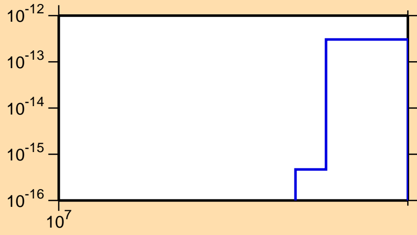
\sigma vs. E for ^{183}\text{Ir} (mt 34)
