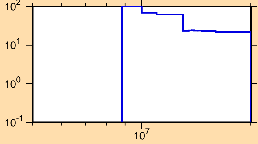
\Delta\sigma/\sigma vs. E for ^{183}\text{Ir}(n,2n)
