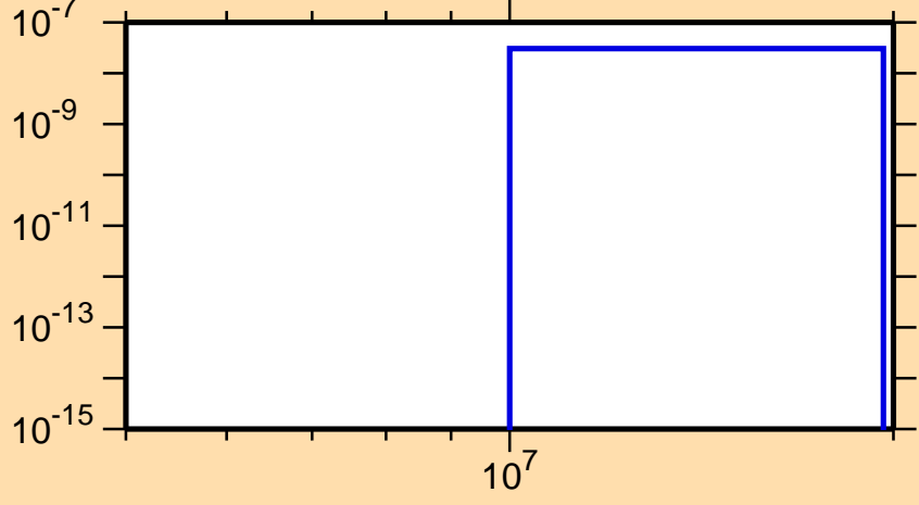
\sigma vs. E for ^{183}\text{Ir}(n,\text{He3})
