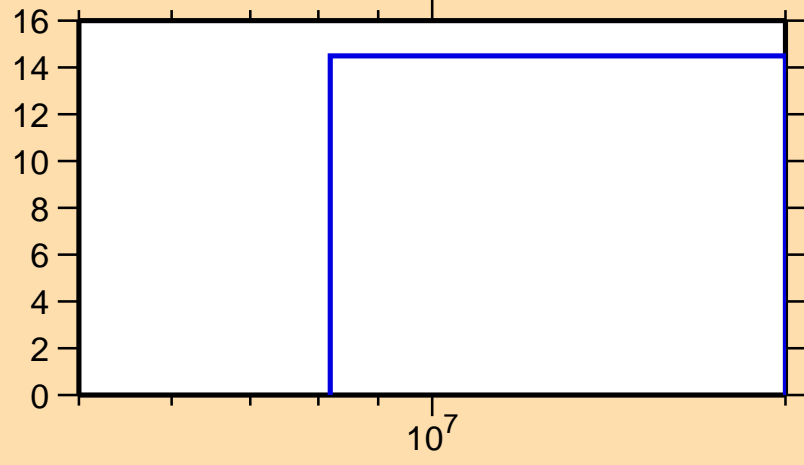
\Delta\sigma/\sigma vs. E for ^{183}\text{Ir}(n,el.)
