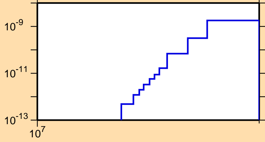
\sigma vs. E for ^{184}\text{Ir}(\text{mt } 45)
