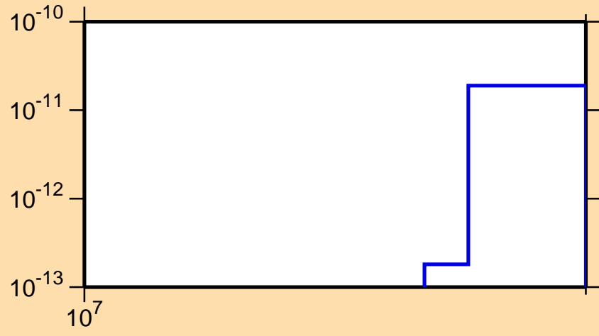
\sigma vs. E for ^{184}\text{Ir} (mt 34)
