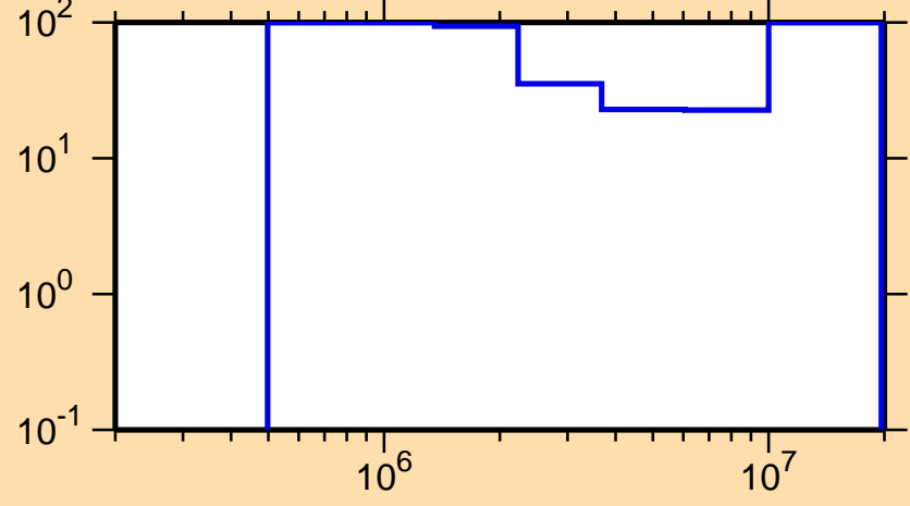
\Delta\sigma/\sigma vs. E for ^{184}\text{Ir}(n,n\text{cont.})
