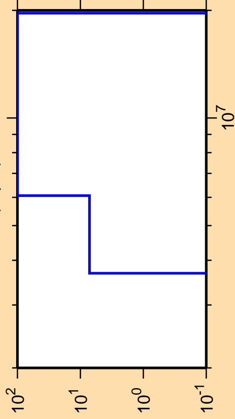
\Delta\sigma/\sigma vs. E for ^{184}\text{Ir}(n,p\alpha)
