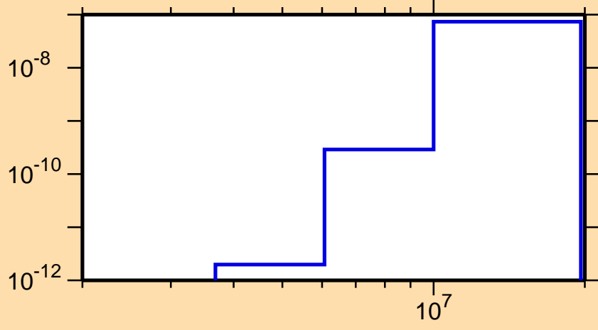
\sigma vs. E for ^{184}\text{Ir}(n,p\alpha)
