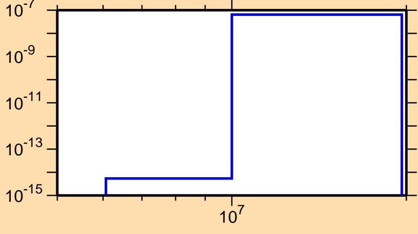
\sigma vs. E for ^{184}\text{Ir}(n,\text{He}3)
