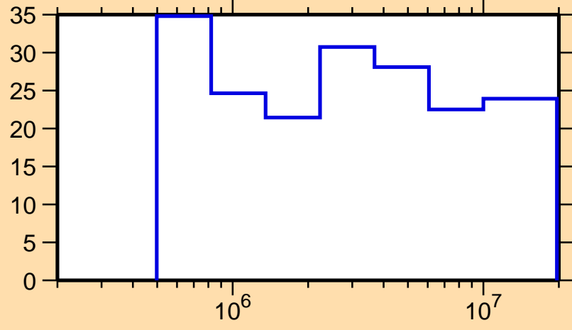
\Delta\sigma/\sigma vs. E for ^{184}\text{Ir}(n,el.)
