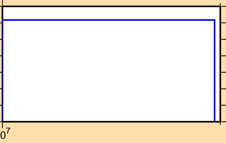
\sigma vs. E for ^{184}\text{Ir}(n,\text{pd})
