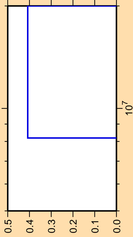
\Delta\sigma/\sigma vs. E for ^{184}\text{Ir}(n,pt)
