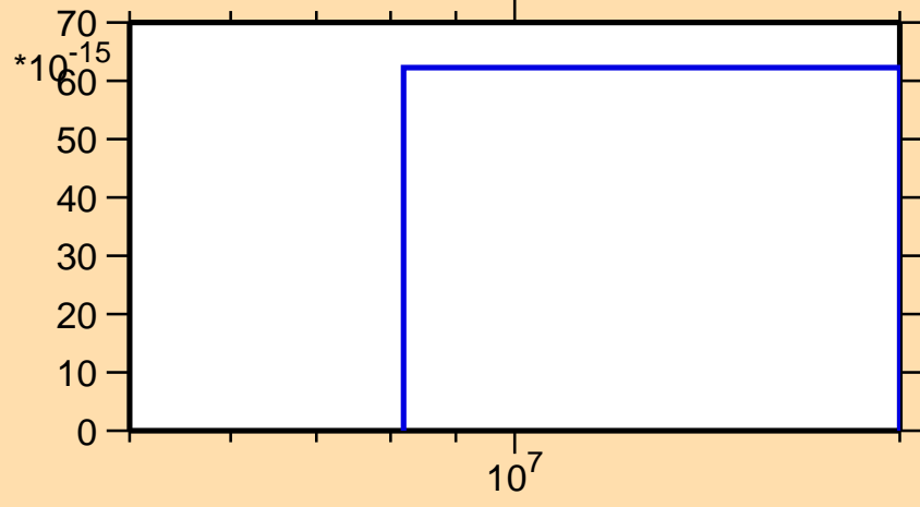
\sigma vs. E for ^{184}\text{Ir}(n,pt)
