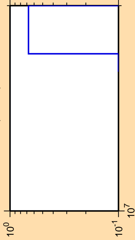
\Delta\sigma/\sigma vs. E for ^{185}\text{Ir} (mt 34)
