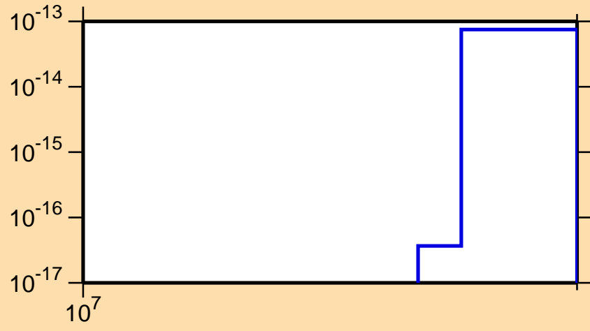
\sigma vs. E for ^{185}\text{Ir} (mt 34)
