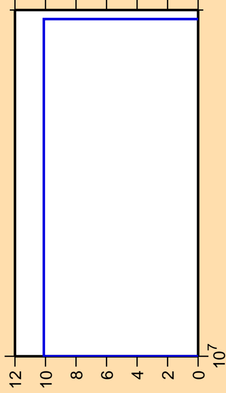
\Delta\sigma/\sigma vs. E for ^{186}\text{Ir} (mt 45)
