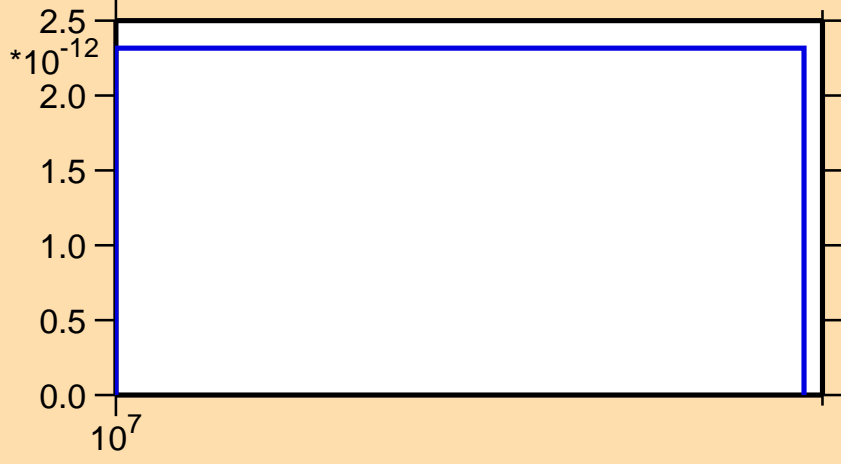
\sigma vs. E for ^{186}\text{Ir} (mt 45)
