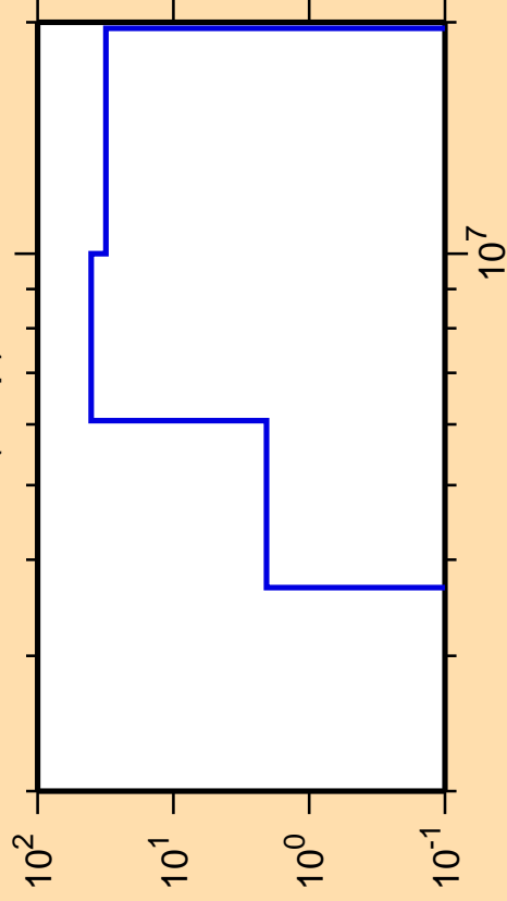
\Delta\sigma/\sigma vs. E for ^{186}\text{Ir}(n,np)
