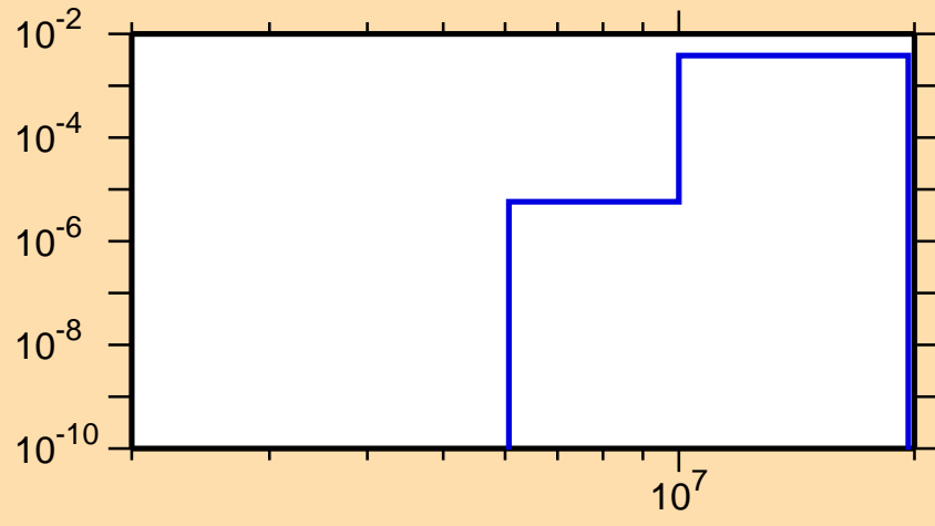
\sigma vs. E for ^{186}\text{Ir}(n,np)
