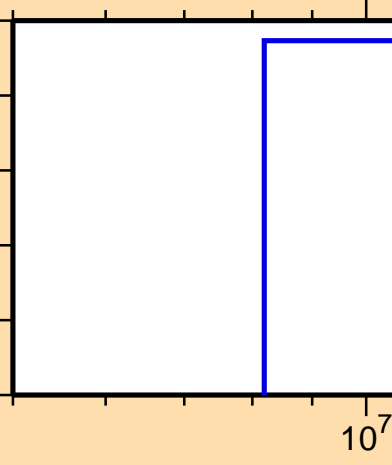
\sigma vs. E for ^{186}\text{Ir}(n,\text{pd})
