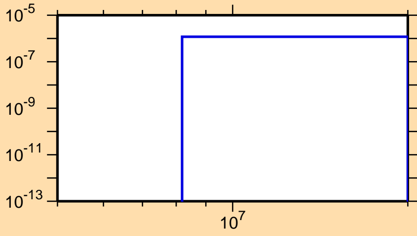
\sigma vs. E for ^{186}\text{Ir}(n,\text{nd})
