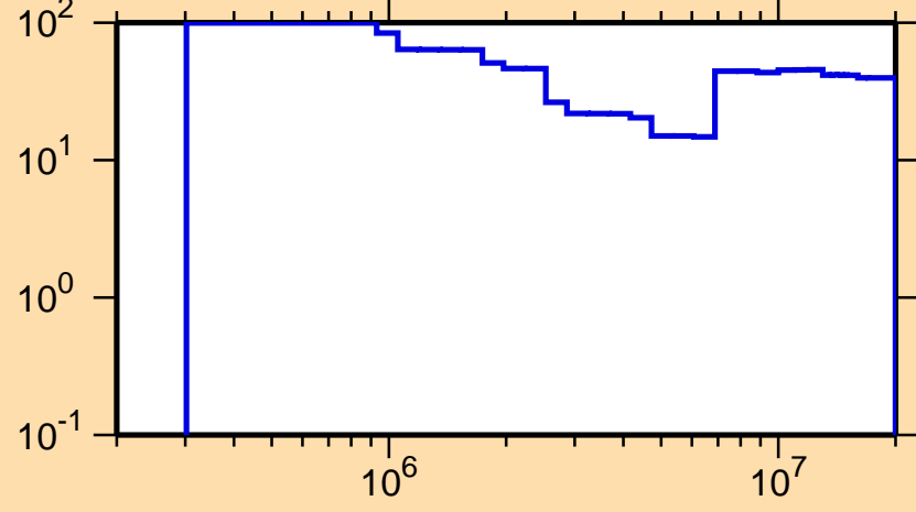
\Delta\sigma/\sigma vs. E for ^{190}\text{Ir}(n,n\text{cont.})
