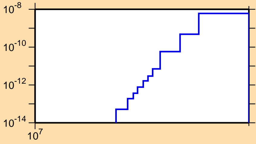
\sigma vs. E for ^{190}\text{Ir}(n,\text{He}3)
