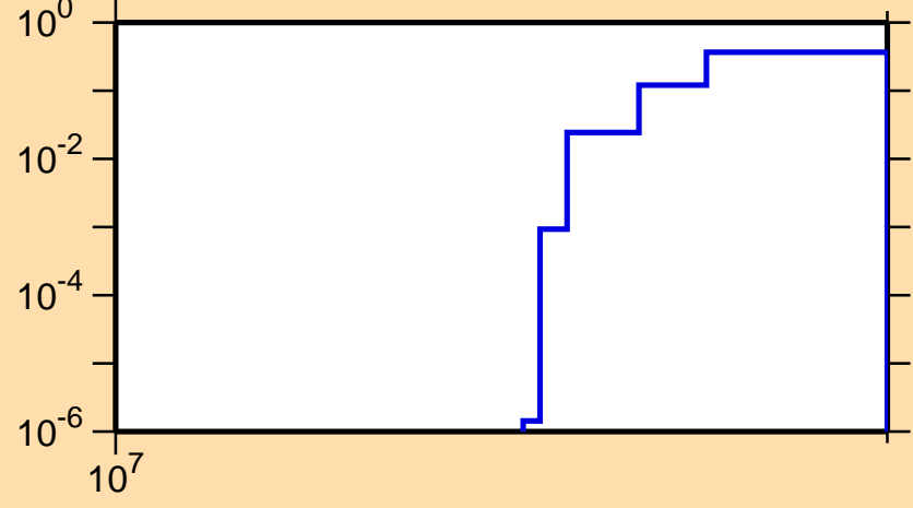
\sigma vs. E for ^{190}\text{Ir}(n,3n)
