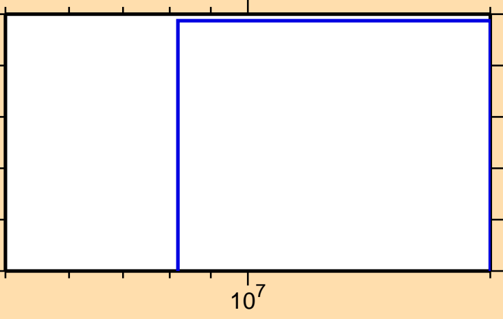
\sigma vs. E for ^{190}\text{Ir}(n,\text{nd})
