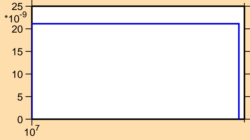
\sigma vs. E for ^{190}\text{Ir}(n,nt)
