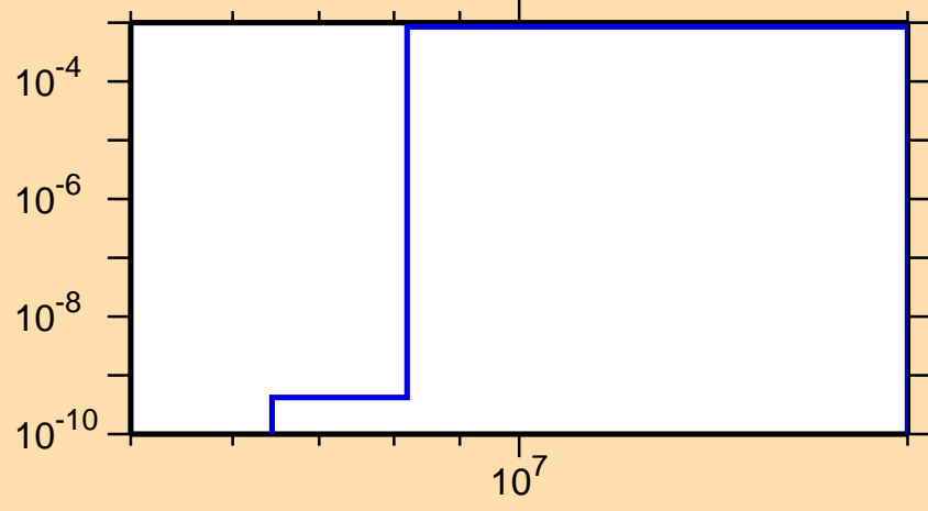
\sigma vs. E for ^{190}\text{Ir}(n,d)
