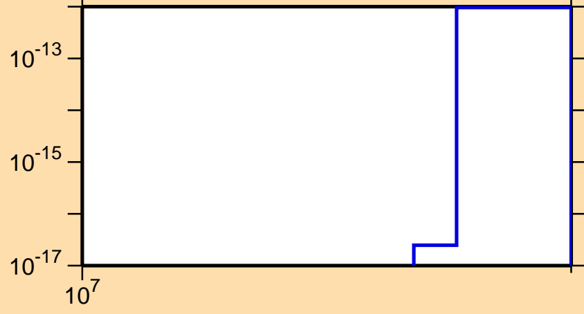
\sigma vs. E for ^{190}\text{Ir}(n,3n\alpha)
