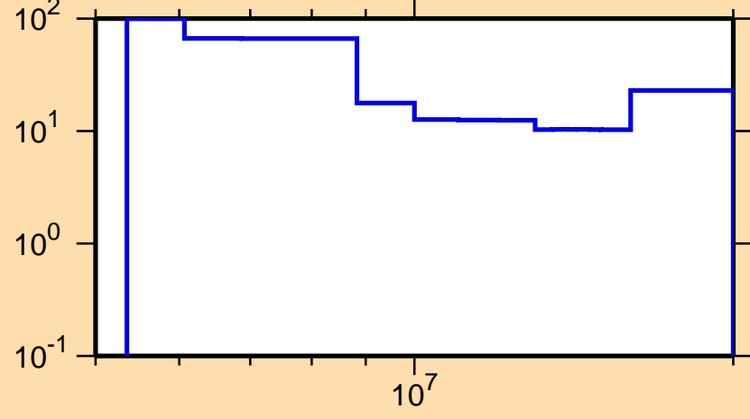
\Delta\sigma/\sigma vs. E for ^{190}\text{Ir}(n,2n)
