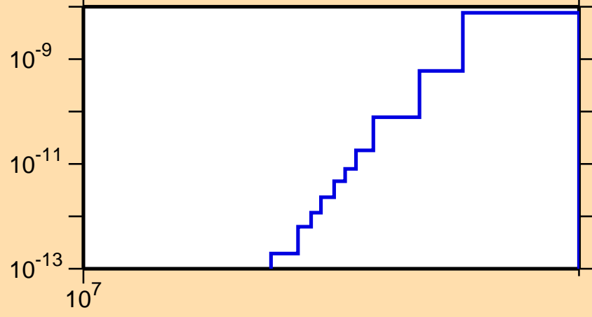
\sigma vs. E for ^{190}\text{Ir}(n,\text{He}3)
