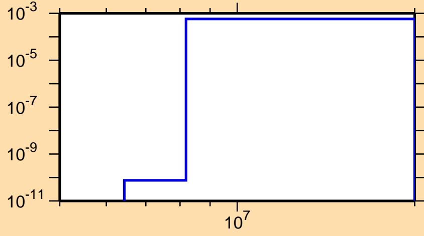
\sigma vs. E for ^{191}\text{Ir}(n,d)
