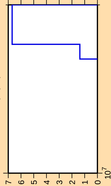
\Delta\sigma/\sigma vs. E for ^{191}\text{Ir}(n,p\alpha)
