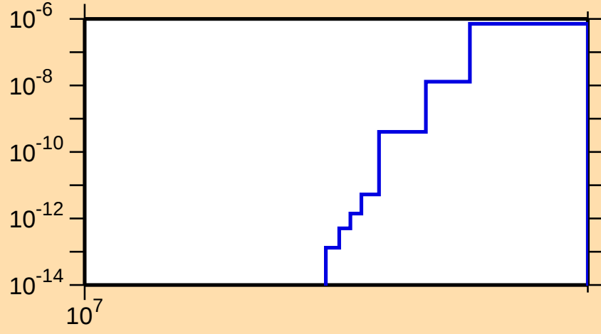
\sigma vs. E for ^{191}\text{Ir}(n,nt)
