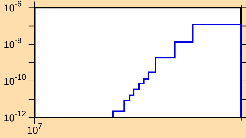
\sigma vs. E for ^{191}\text{Ir}(n,2n\alpha)
