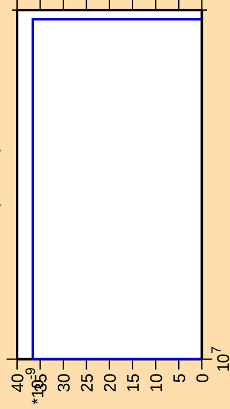
\Delta\sigma/\sigma vs. E for ^{191}\text{Ir}(\text{mt } 42)
