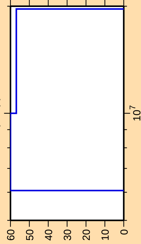
\Delta\sigma/\sigma vs. E for ^{191}\text{Ir}(n,np)
