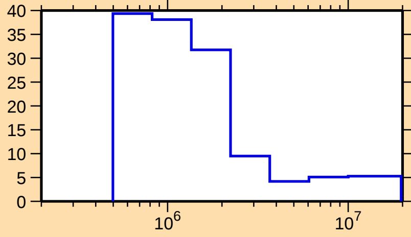
\Delta\sigma/\sigma vs. E for ^{191}\text{Ir}(n,n\text{oncl.})
