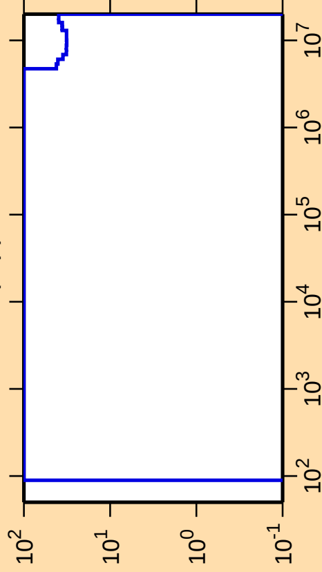
\Delta\sigma/\sigma vs. E for ^{191}\text{Ir}(n,p)
