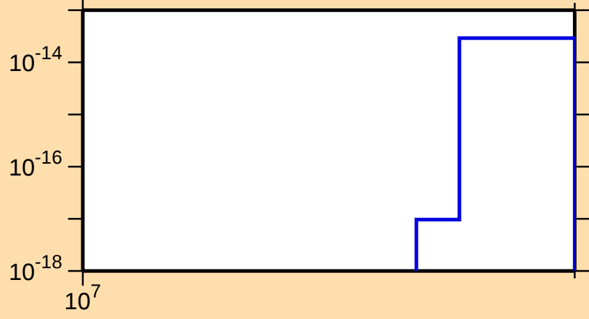
\sigma vs. E for ^{191}\text{Ir}(\text{mt } 34)
