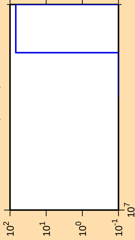
\Delta\sigma/\sigma vs. E for ^{191}\text{Ir}(\text{mt 11})
