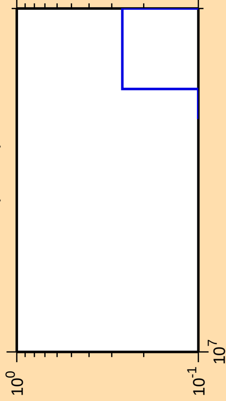
\Delta\sigma/\sigma vs. E for ^{191}\text{Ir}(\text{mt } 34)
