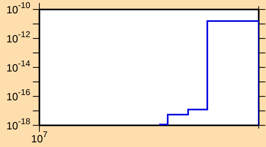
\sigma vs. E for ^{191}\text{Ir}(\text{mt 11})
